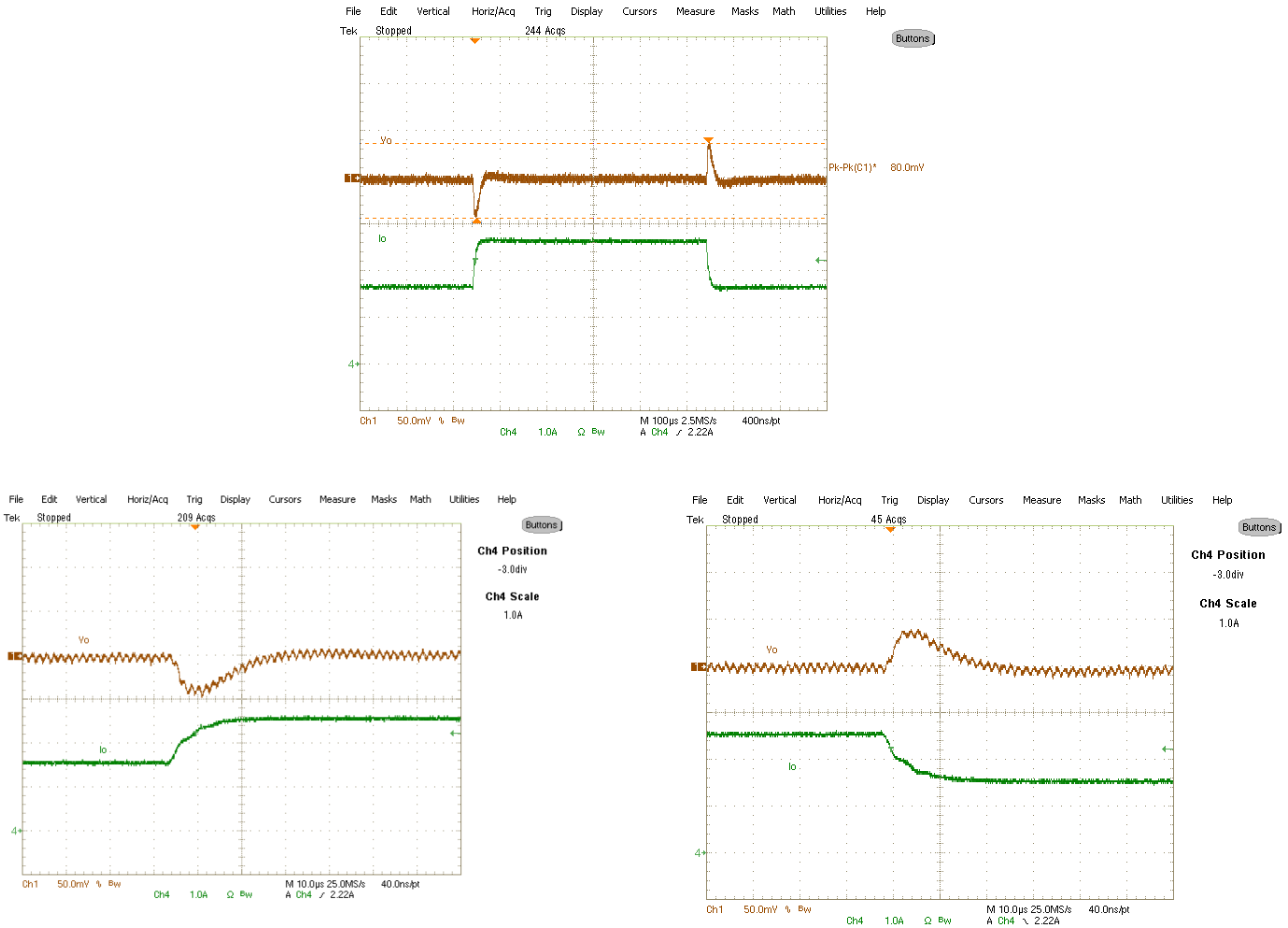
Fig. 23. Transient Response, 1A to 2A step 2.5A/μs Ch 1 :V o , Ch 4 :I o
