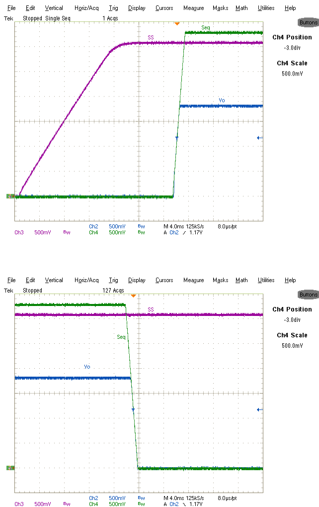
Fig. 18: Simultaneous Tracking a 3.3V input at power-up and shut-down Ch2: Vout Ch3:SS Ch4: Seq
