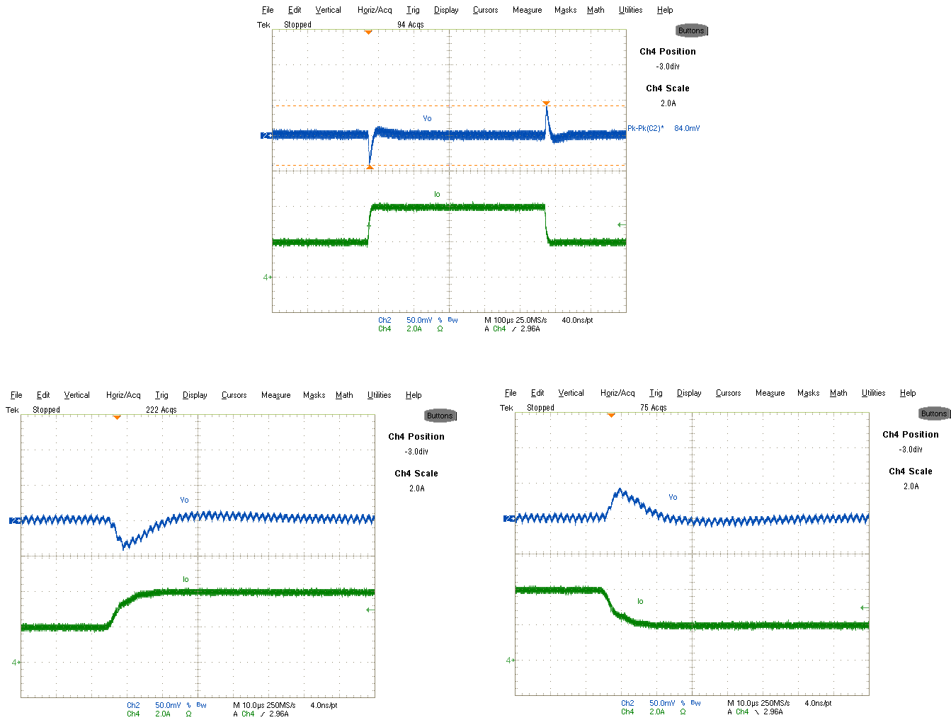
Fig. 23. Transient Response, 2A to 4A step 2.5A/ \mu s Ch 2 :V o , Ch 4 :I o
