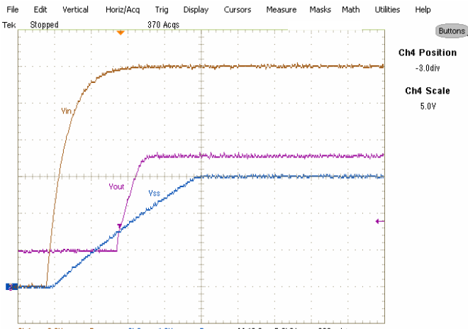
Fig. 9: Pre-Bias Start up, 0A Load Ch 1 :V in , Ch 2 :V SS , Ch 3 :V out
