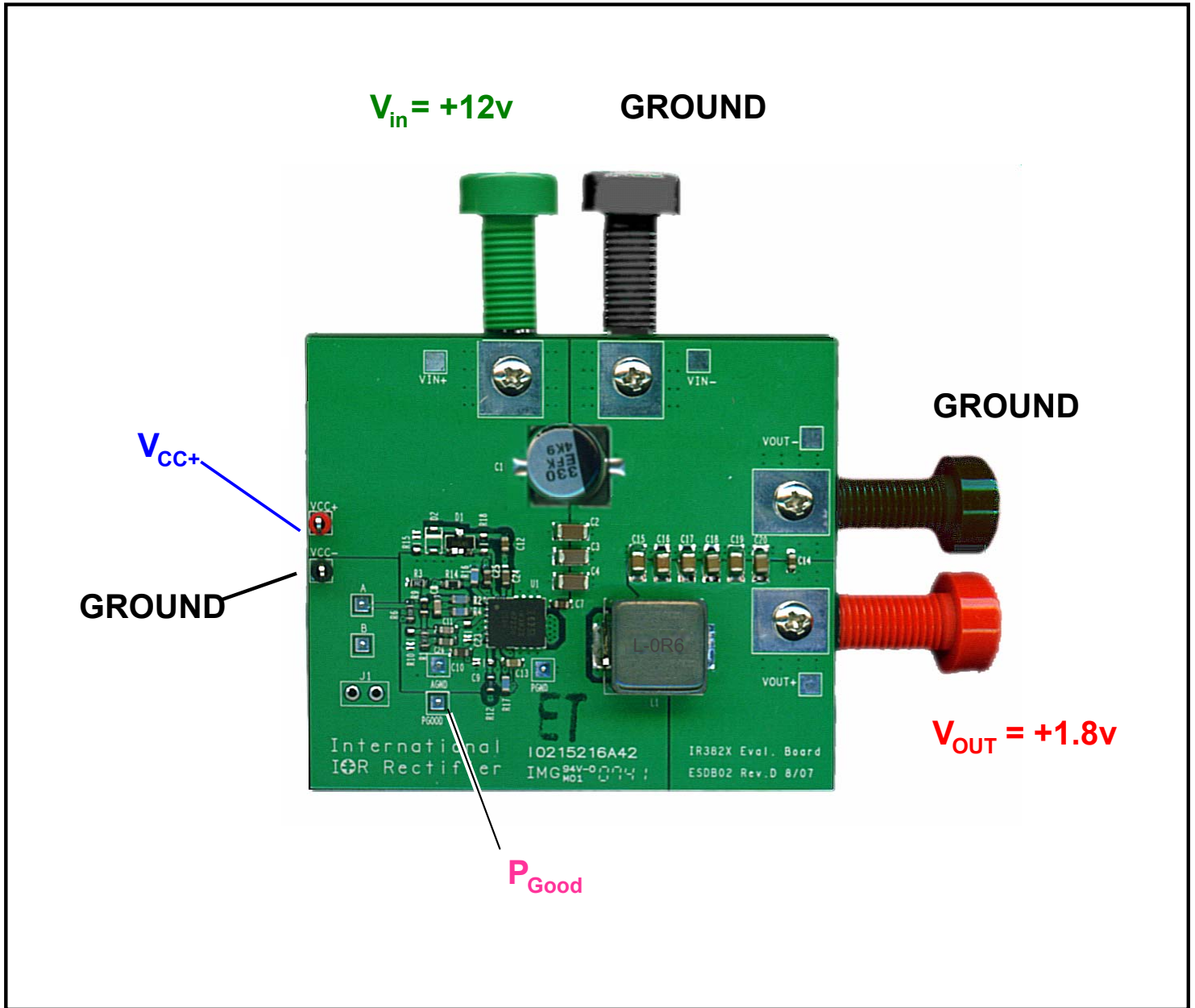
Fig. 1: Connection diagram of IR3820 evaluation board
