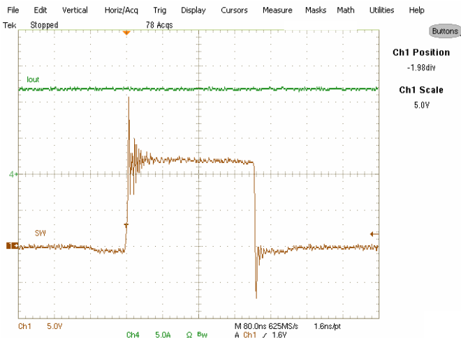
Fig. 11: Inductor node at 12A load Ch 1 :LX, Ch 4 :I out
