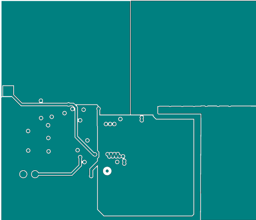
Fig. 4: Board layout, mid-layer I
