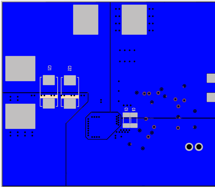
Fig. 3: Board layout, bottom overlay (rear view)
