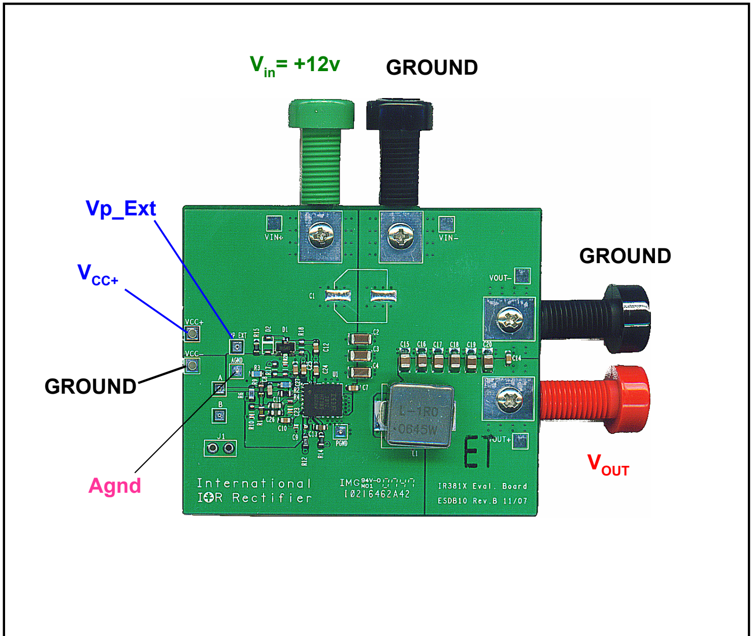
Fig. 1: Connection diagram of IR3812 evaluation board
