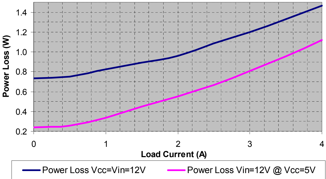
Fig.16: Power loss versus load current
