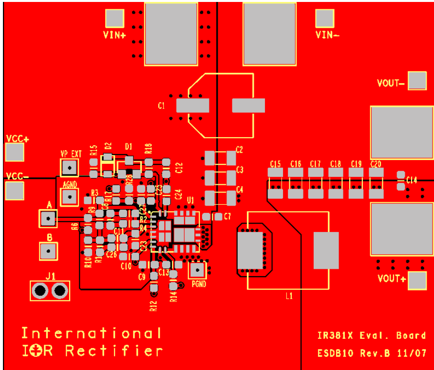
Fig. 2: Board layout, top overlay
