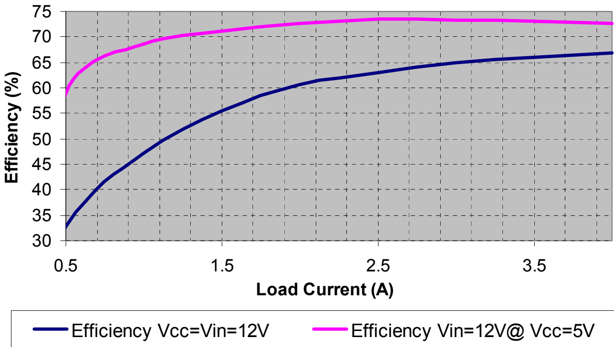
Fig.15: Efficiency versus load current
