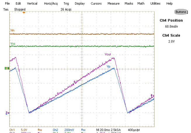
Fig. 8: Tracking Operation V_p: 0-0.6V , 4A Load Ch_1: V_{in} , Ch_2: V_p , Ch_3: V_{out} , Ch_4: V_{ss}
