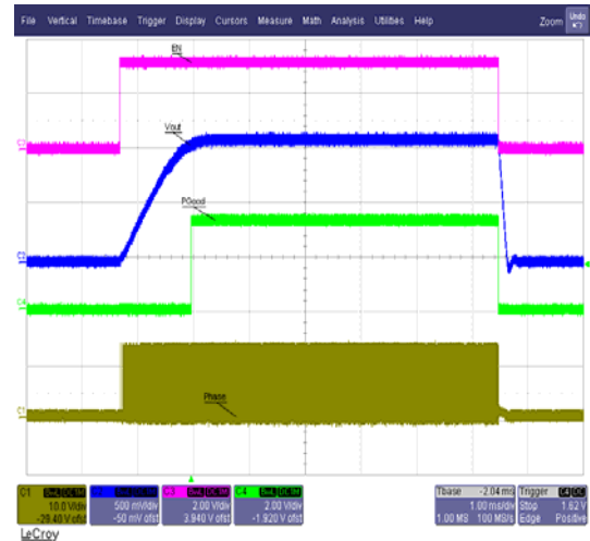
Ch1-Phase Voltage (10V/Div) Ch2-Vout(500mV/Div) Ch3-EN(2V/Div) Ch4-PGood(2V/Div)
