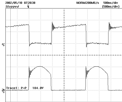
Figure 17 – 36 VDC, Full Load. Upper Trace: I_{DRAIN} , 1 A/div. Lower Trace: V_{DRAIN} , 50 V/div, 500 ns/div.
