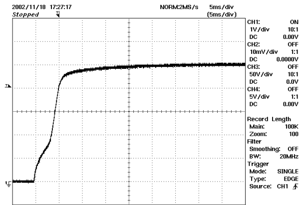
Figure 21 – Start-up Profile, 36 VDC, Zero Load. 1 V/div, 5 ms/div.
