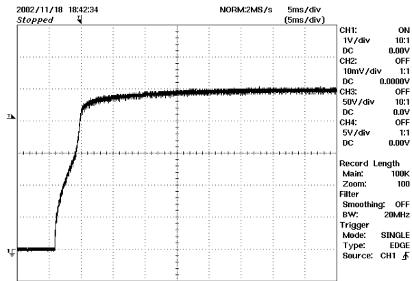
Figure 25 – Start-up Profile, 72 VDC, Zero Load, 1 V/div, 5 ms/div.
