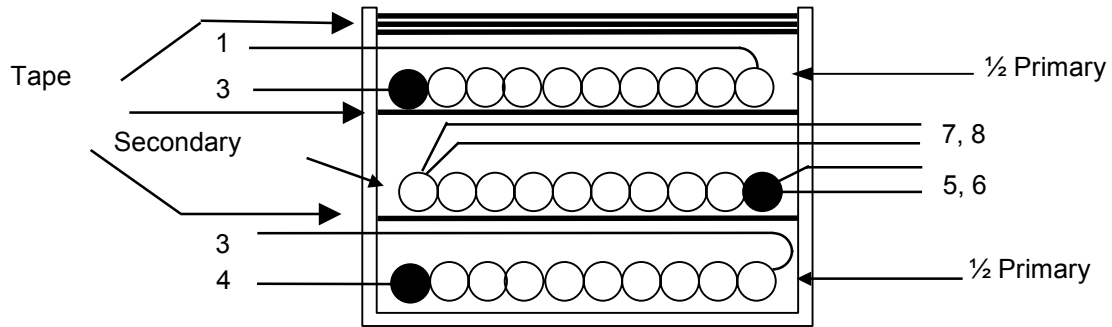
Figure 5 – EP-21 Transformer Build Diagram.
