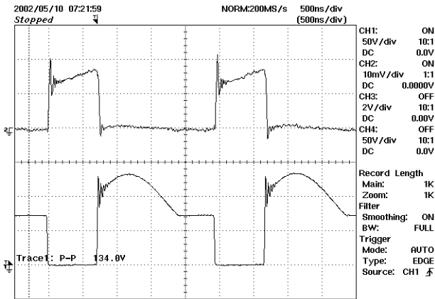
Figure 17 – 36 VDC, Full Load. Upper Trace: I_{DRAIN} , 1 A/div. Lower Trace: V_{DRAIN} , 50 V/div, 500 ns/div.
