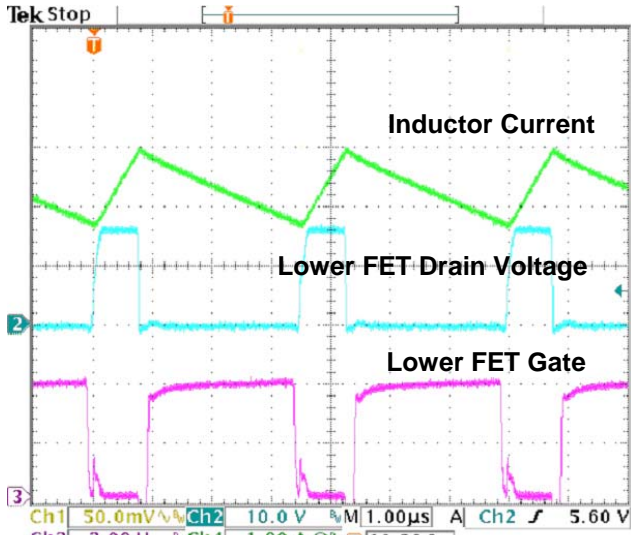
Figure 2 – Phase 2 FET Gates & Output
