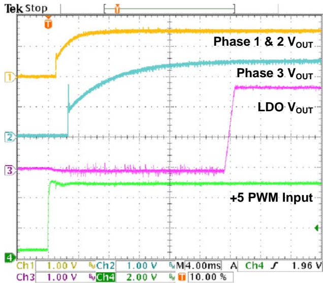
Figure 5 – Start-Up Sequence
