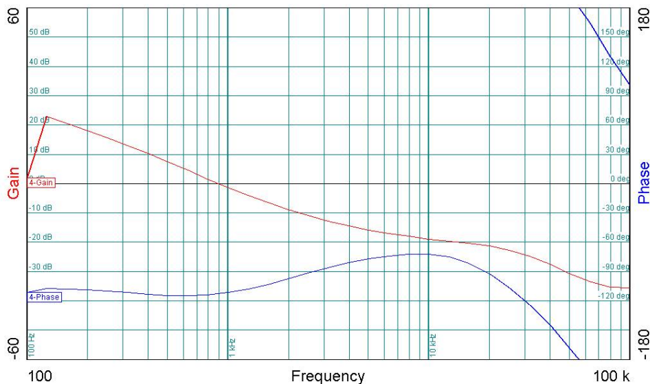
Figure 26 - Gain-Phase Plot, 36 VDC, Light Load (100 mA). Vertical Scale: Gain = 10 dB / div, Phase = 30° / div. Crossover Frequency = 0.9 kHz, Phase Margin = 65°
