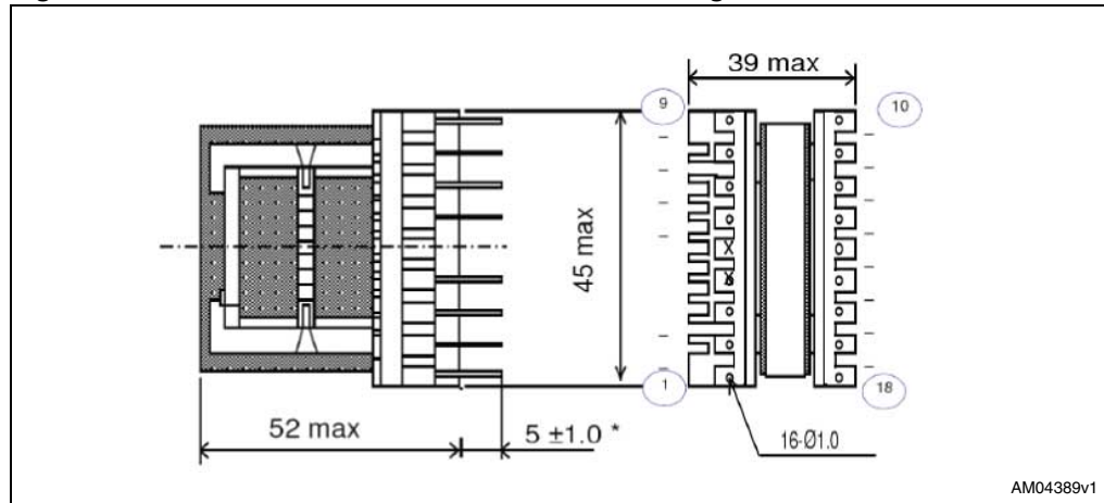
Figure 4. Resonant transformer: mechanical drawing
