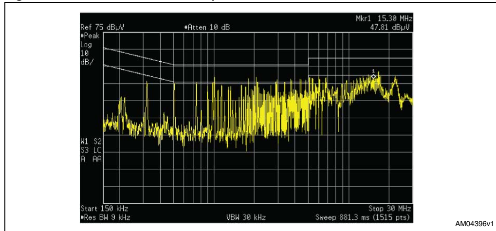
Figure 12. Conducted emissions - neutral - V_{in} = 230\ \text{Vac} , I_{out} = 6\ \text{A}
