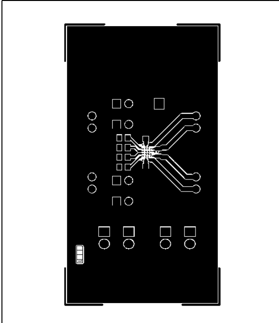
Figure 4. PCB middle layer 2
