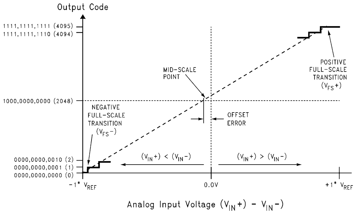
FIGURE 1. Transfer Characteristic
