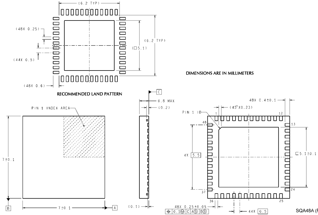
48-Lead LLP Package Ordering Number ADC11C170CISQ NS Package Number SQA48A
