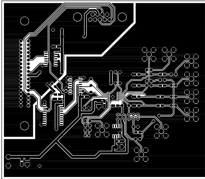
Fig. 23. The Evaluation Board Component Side Artwork
