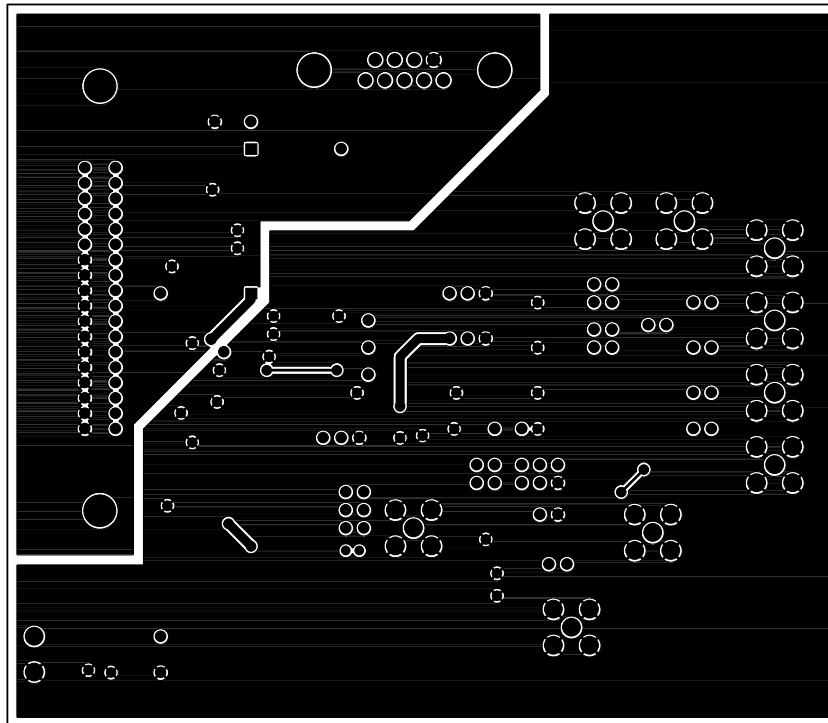
Fig. 23. The Evaluation Board SolderSide Artwork
