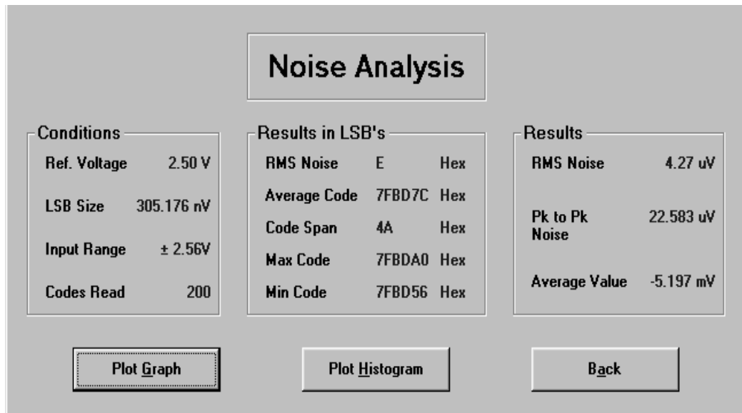
Fig. 6. The ADC Noise Analysis Screen
