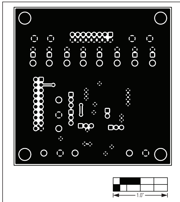
Figure 31. MAX11615 EV Kit Daughter Board PCB Layout—Bottom
