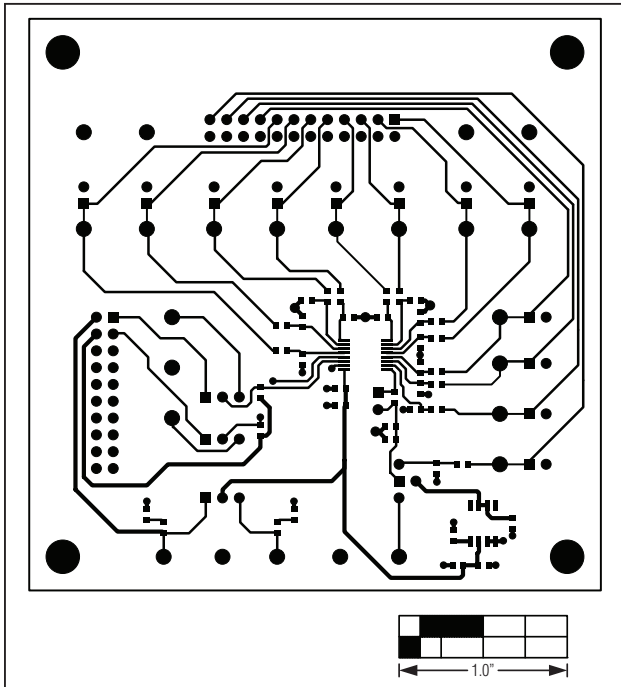
Figure 34. MAX11616 EV Kit Daughter Board PCB Layout—Top
