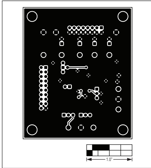
Figure 23. MAX11613 EV Kit Daughter Board PCB Layout—Bottom
