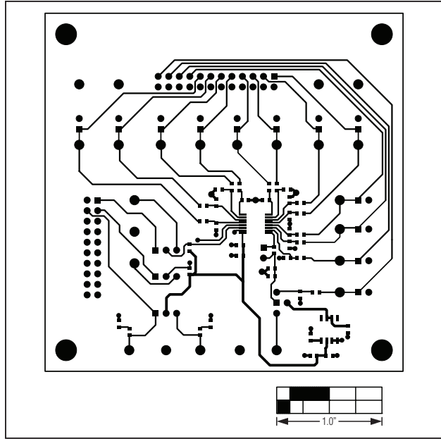
Figure 38. MAX11617 EV Kit Daughter Board PCB Layout—Top
