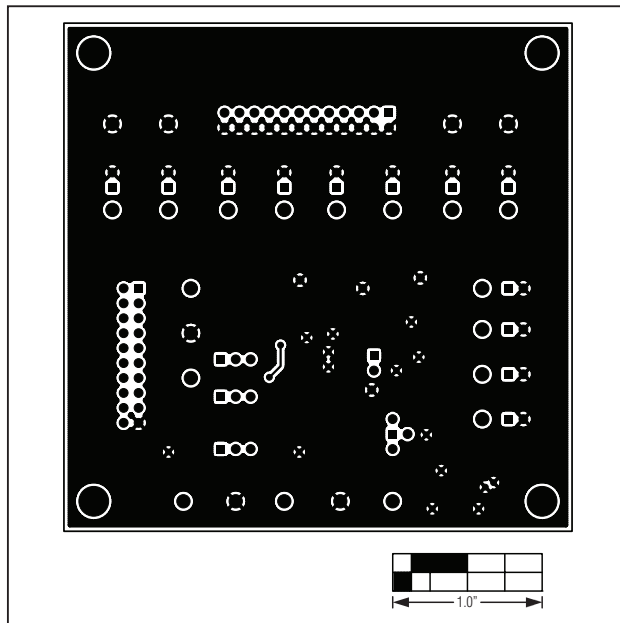
Figure 39. MAX11617 EV Kit Daughter Board PCB Layout—Bottom
