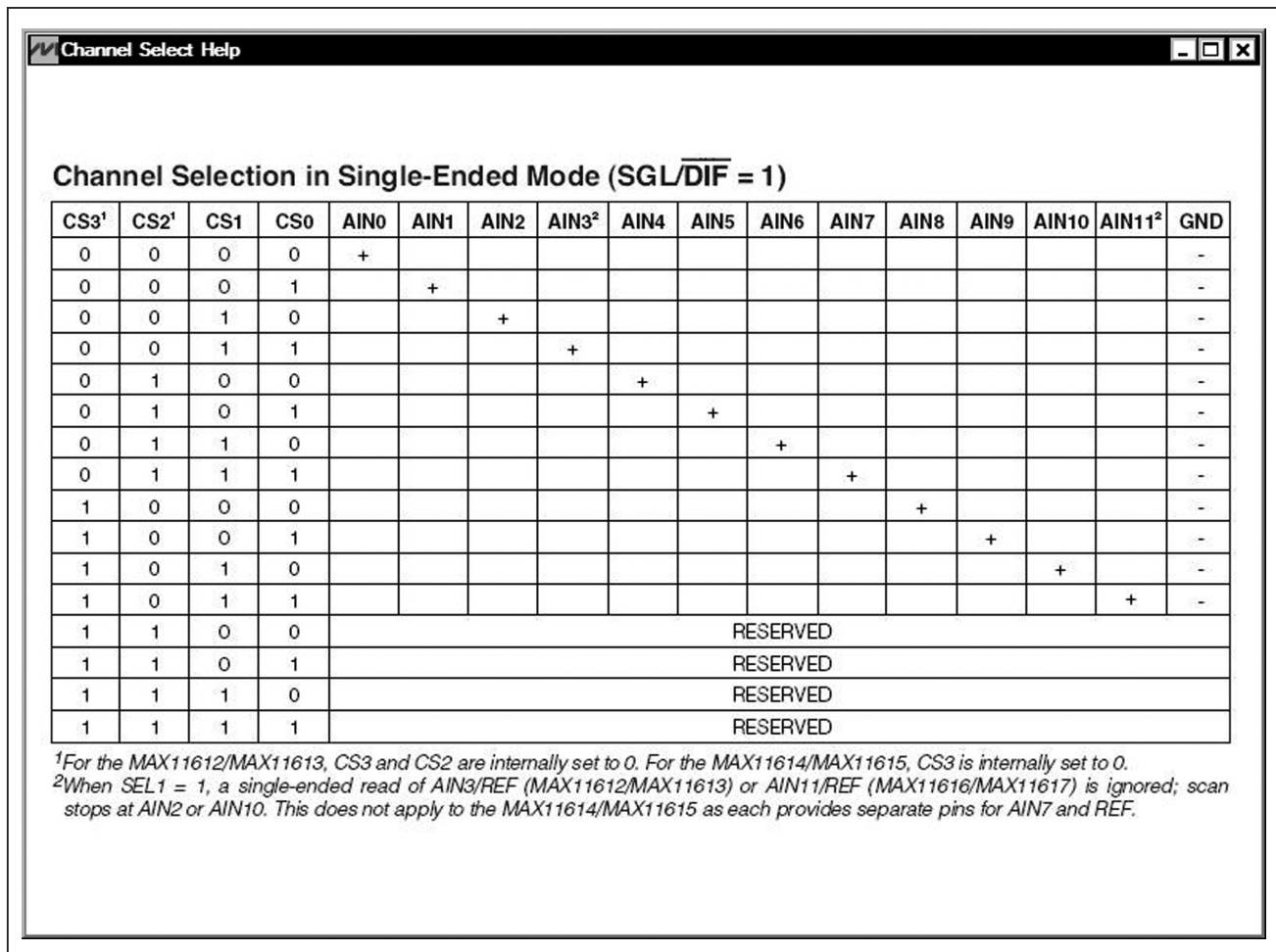
Figure 3. Channel-Selection Reference Table
