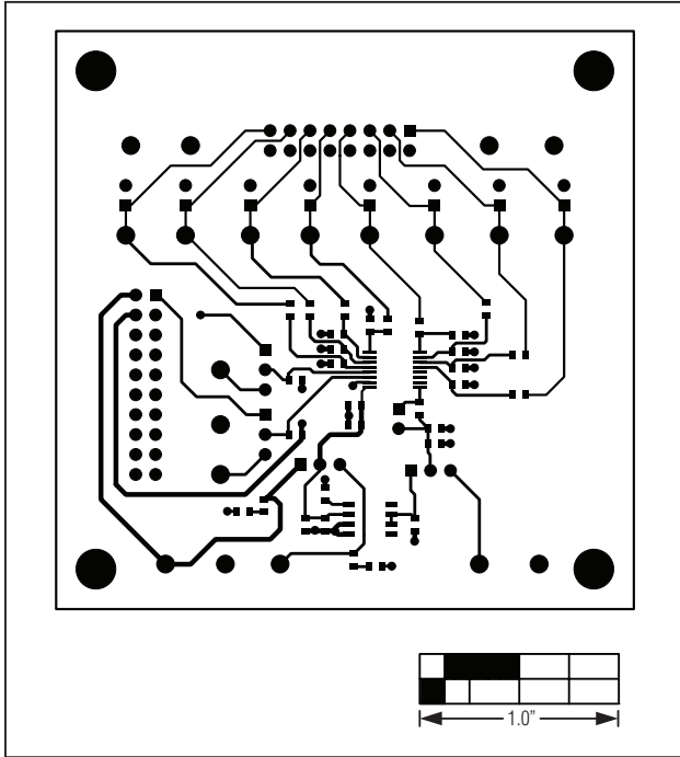
Figure 26. MAX11614 EV Kit Daughter Board PCB Layout—Top
