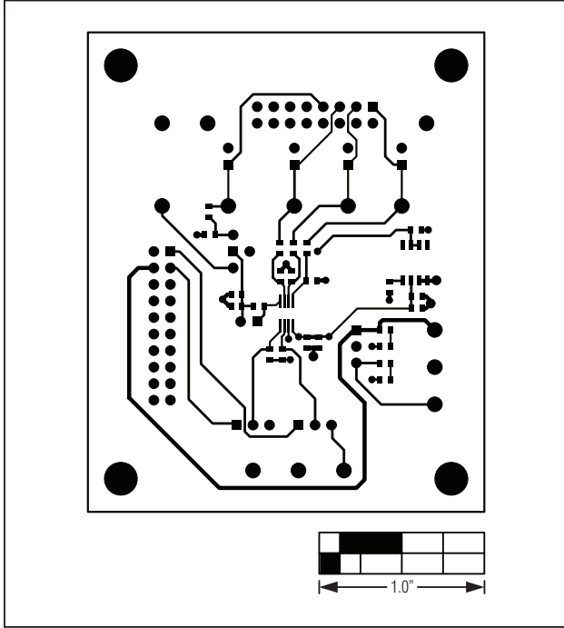
Figure 22. MAX11613 EV Kit Daughter Board PCB Layout—Top
