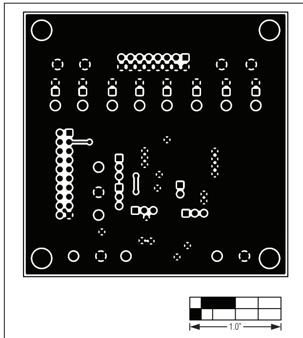
Figure 27. MAX11614 EV Kit Daughter Board PCB Layout—Bottom
