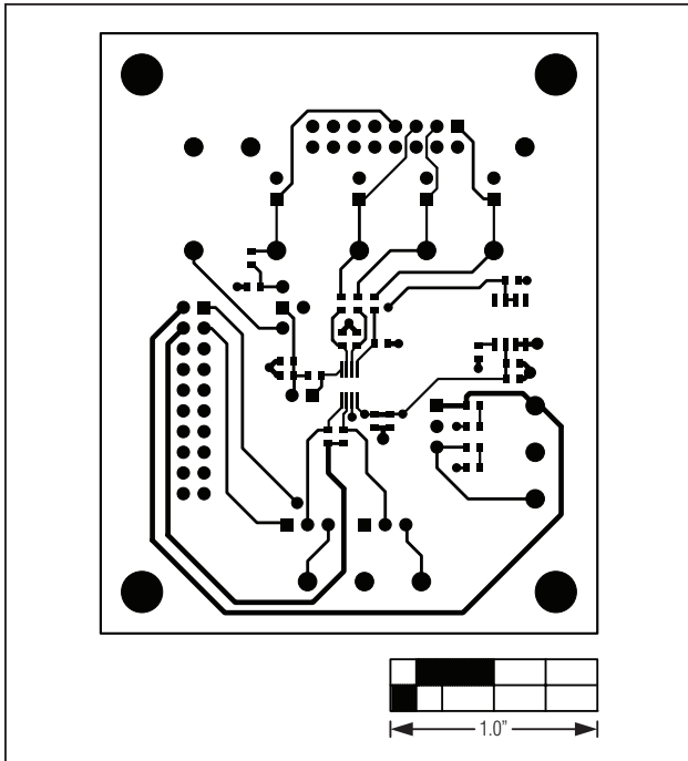
Figure 18. MAX11612 EV Kit Daughter Board PCB Layout—Top
