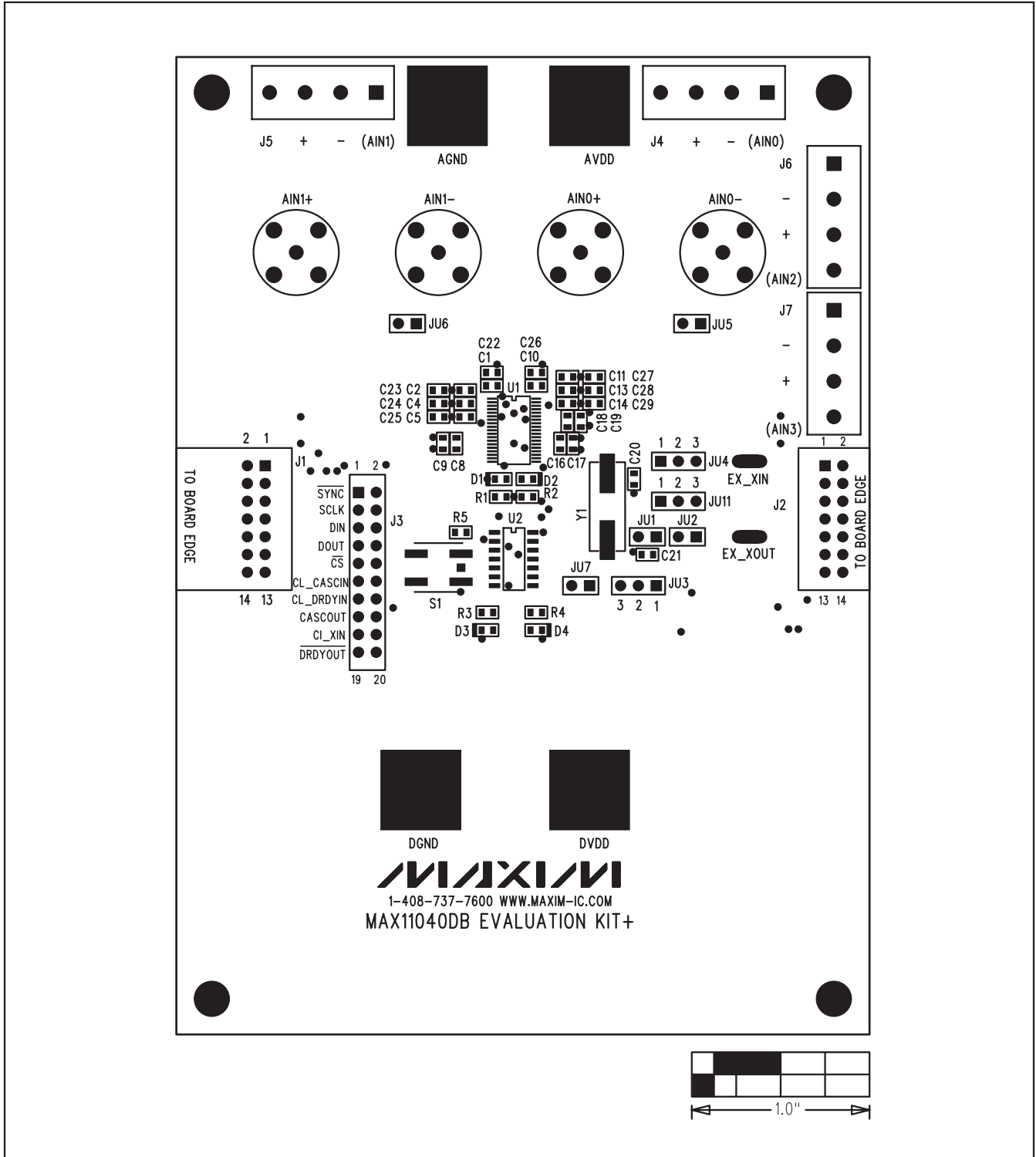
Figure 12. MAX11040 Daughterboard Component Placement Guide—Top
