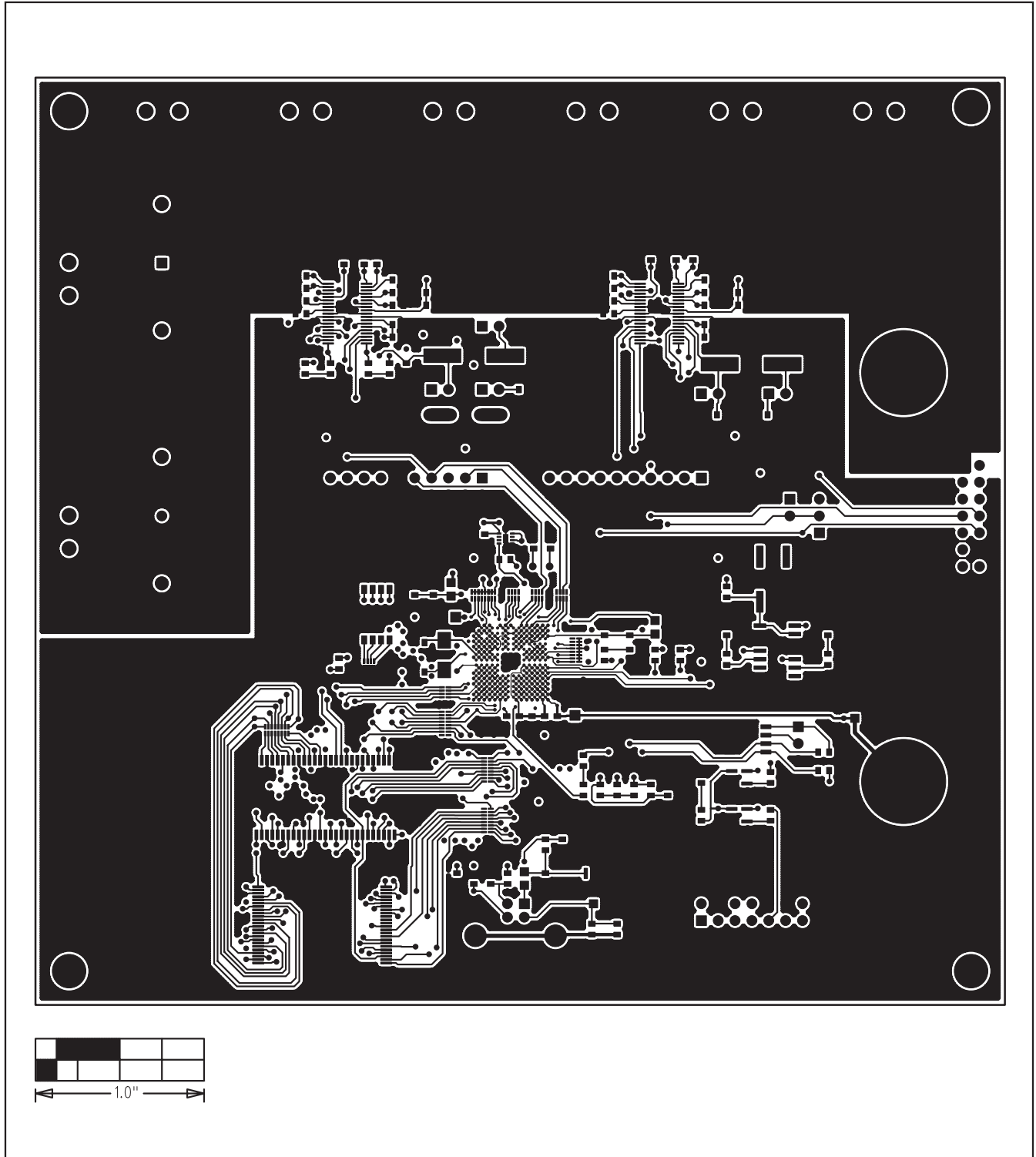
Figure 4. MAX11040 EV Kit PCB Layout—Component Side
