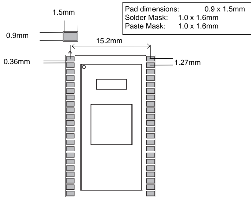
Figure 29 Application board footprint
