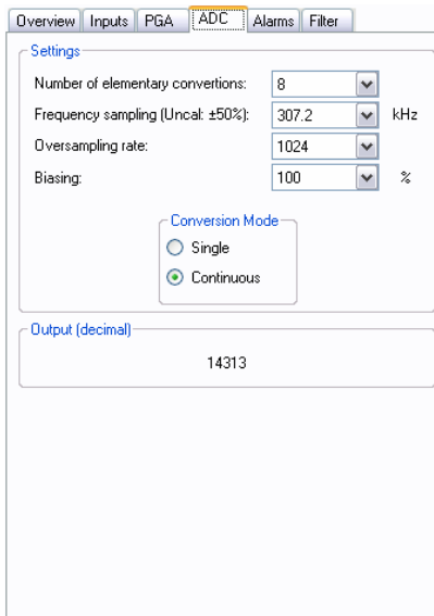
Figure 16 "ADC" sub tab
