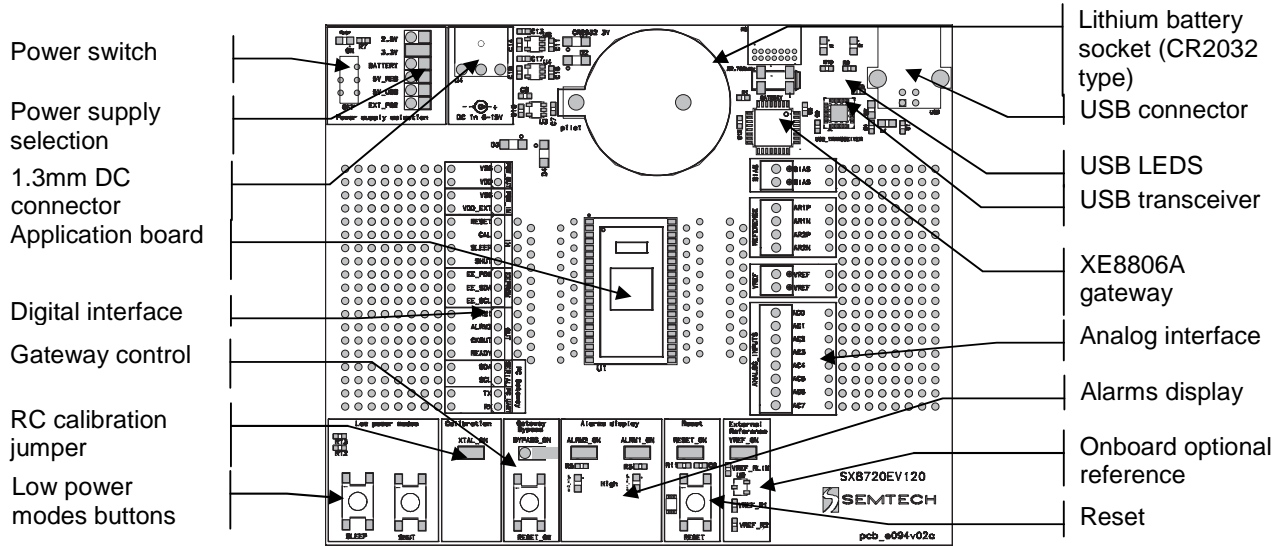
Figure 7 XE8000EV120 board overview
