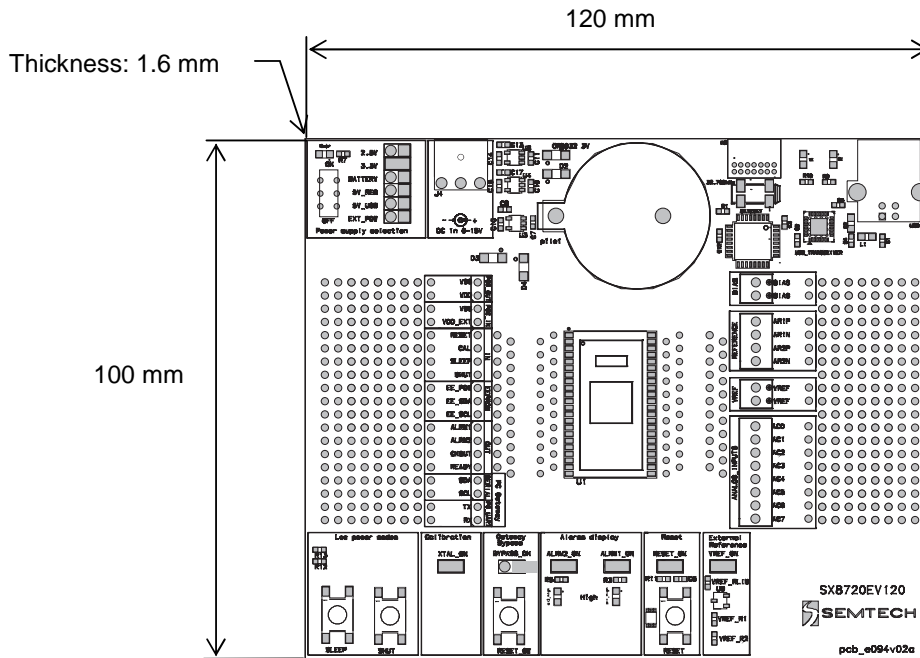
Figure 26 XE8000EV120 physical dimensions
