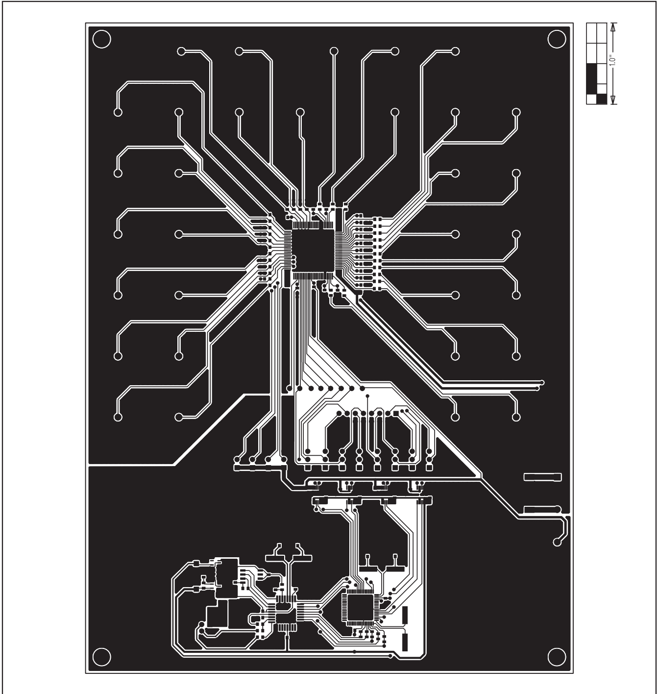
Figure 5. MAX9675 EV Kit PCB Layout—Component Side
