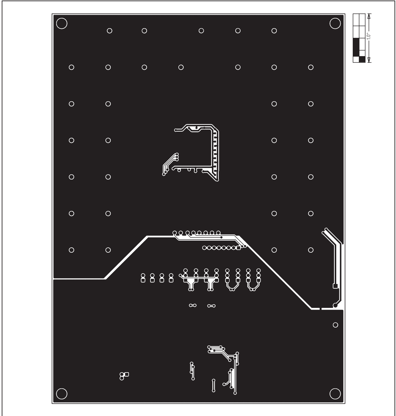
Figure 6. MAX9675 EV Kit PCB Layout—Solder Side
