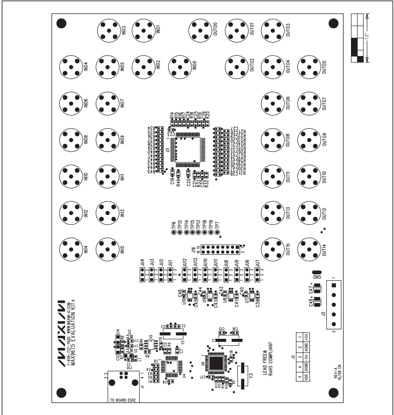
Figure 4. MAX9675 EV Kit Component Placement Guide—Component Side
