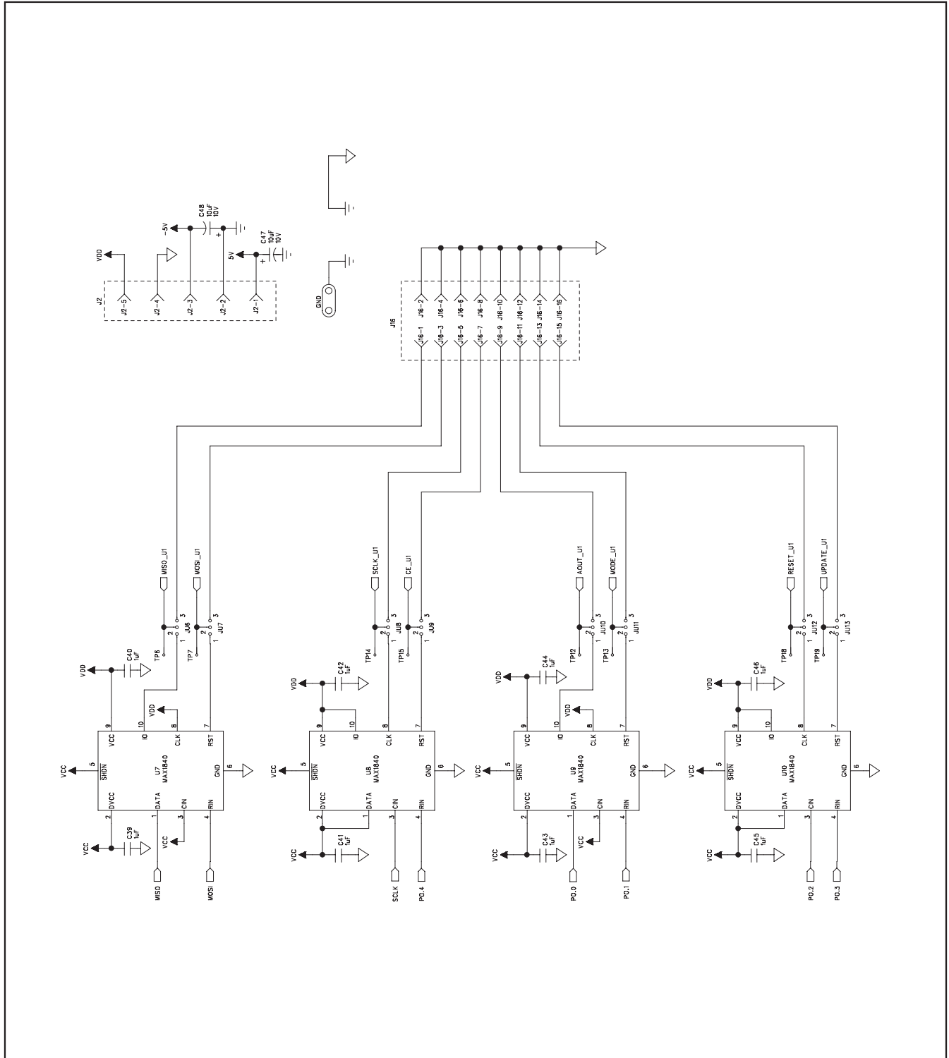
Figure 3b. MAX9675 EV Kit Schematic (Sheet 2 of 3)
