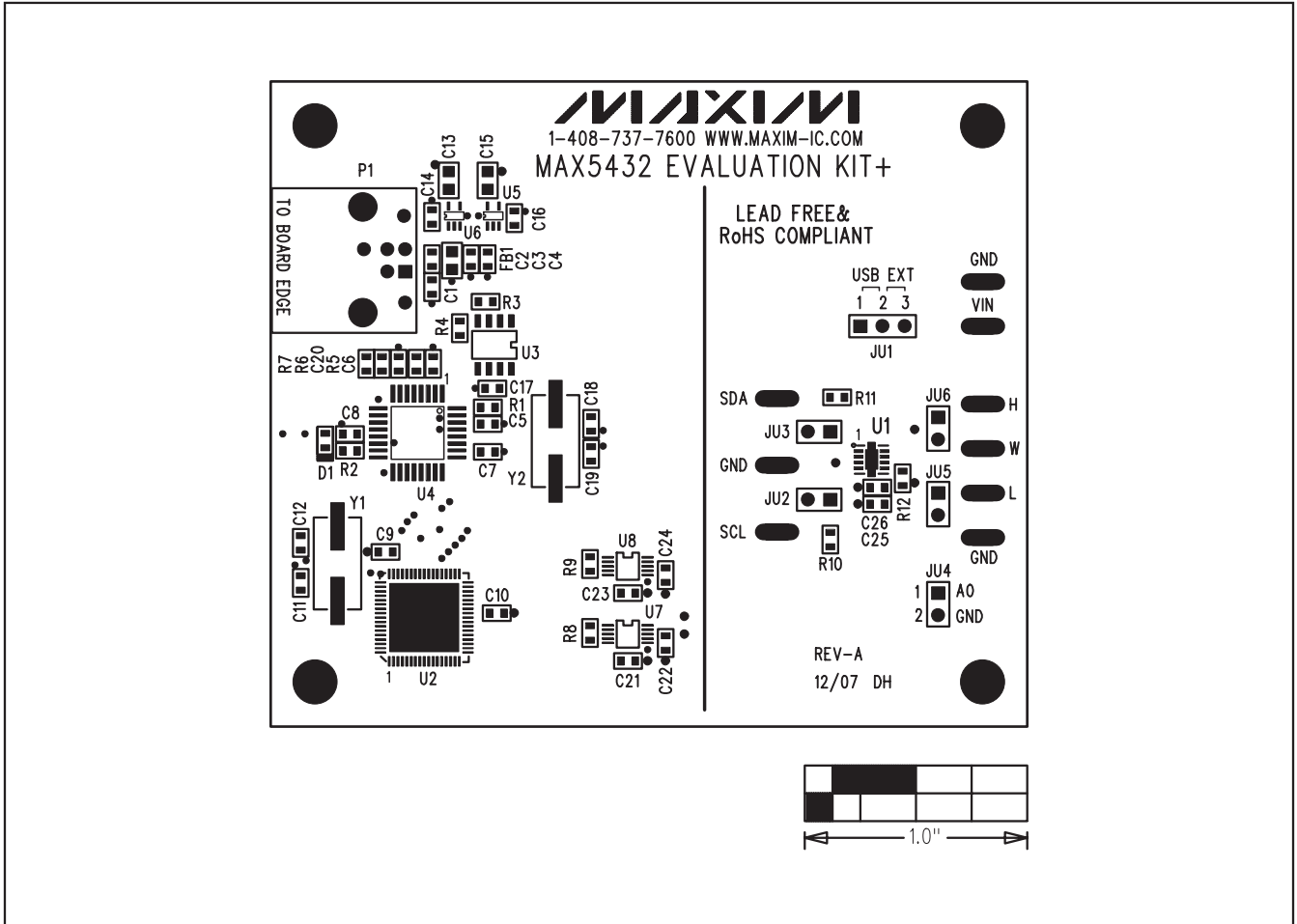
Figure 5. MAX5432 EV Kit Component Placement Guide—Component Side
