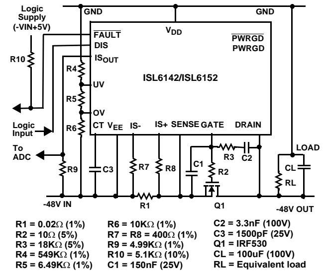
FIGURE 4. TYPICAL APPLICATION
