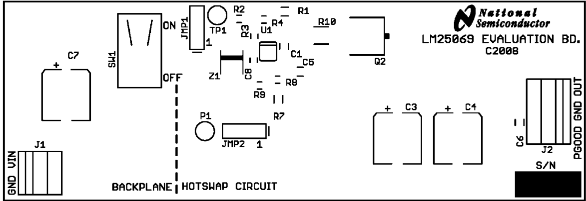
Board Silkscreen
