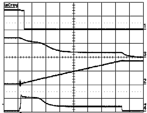
FIGURE 10. Turn-On Sequence into a 4 \Omega Load
