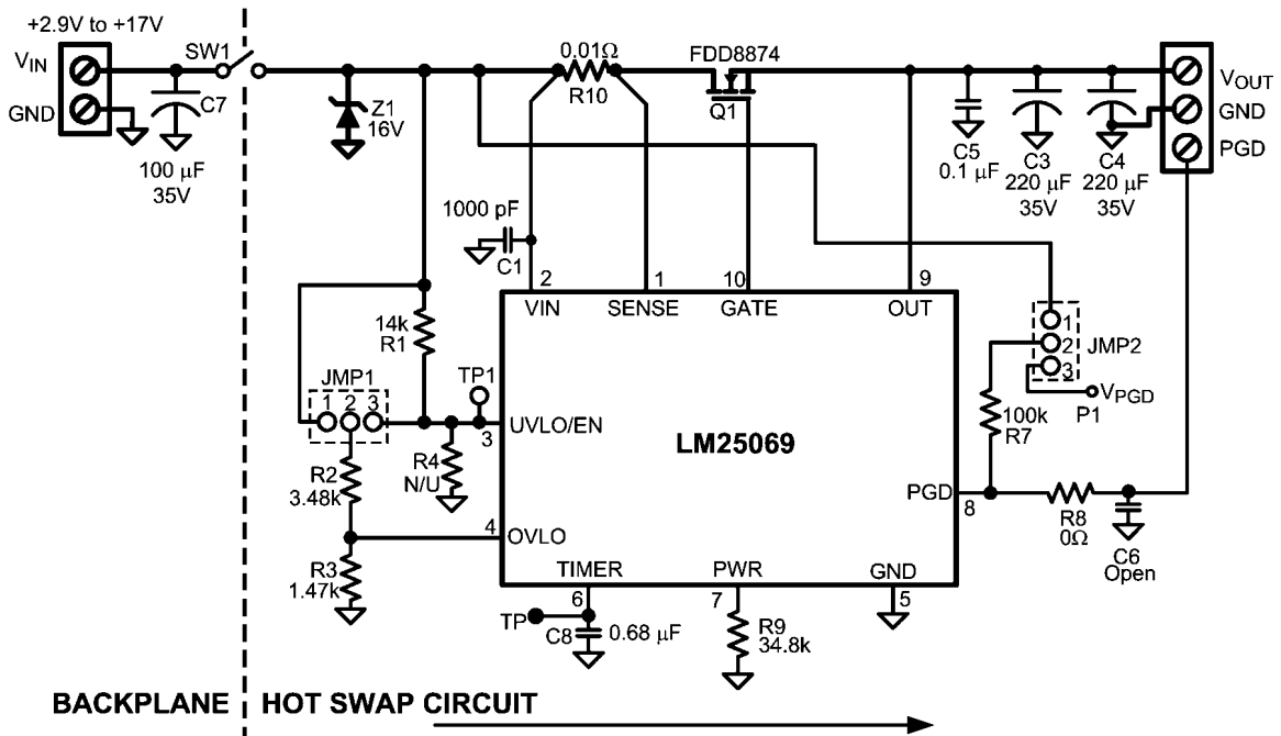
FIGURE 2. Evaluation Board Schematic
