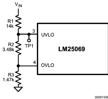
FIGURE 5. UVLO, OVLO Inputs (Option A)
