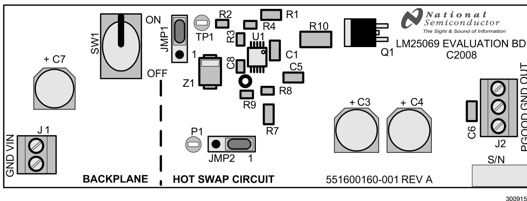
FIGURE 1. Evaluation Board - Top Side
