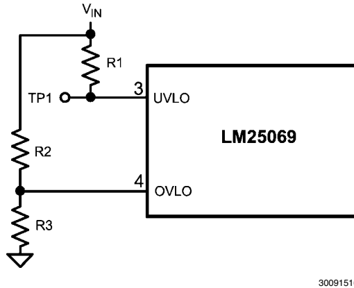
FIGURE 7. Minimum UVLO Threshold, Adjustable OVLO
