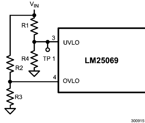
FIGURE 6. UVLO, OVLO Inputs (Option B)
