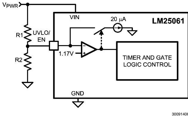
FIGURE 5. Programming the UVLO Threshold
