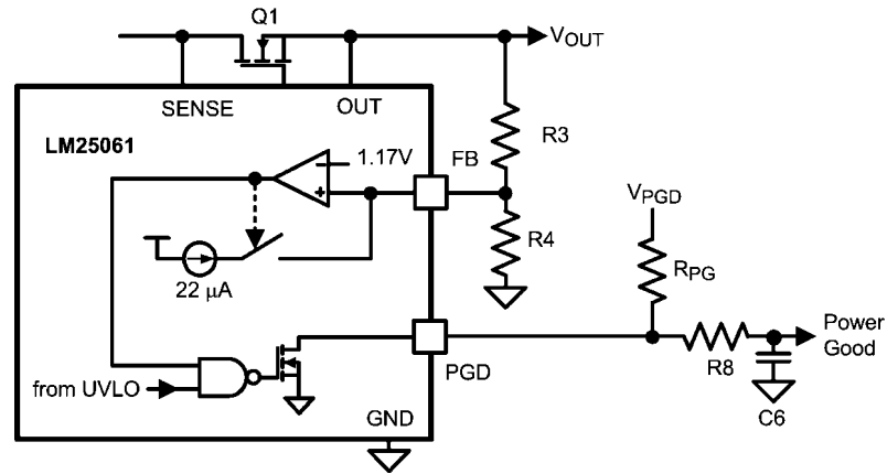
FIGURE 7. Programming the PGD Threshold
