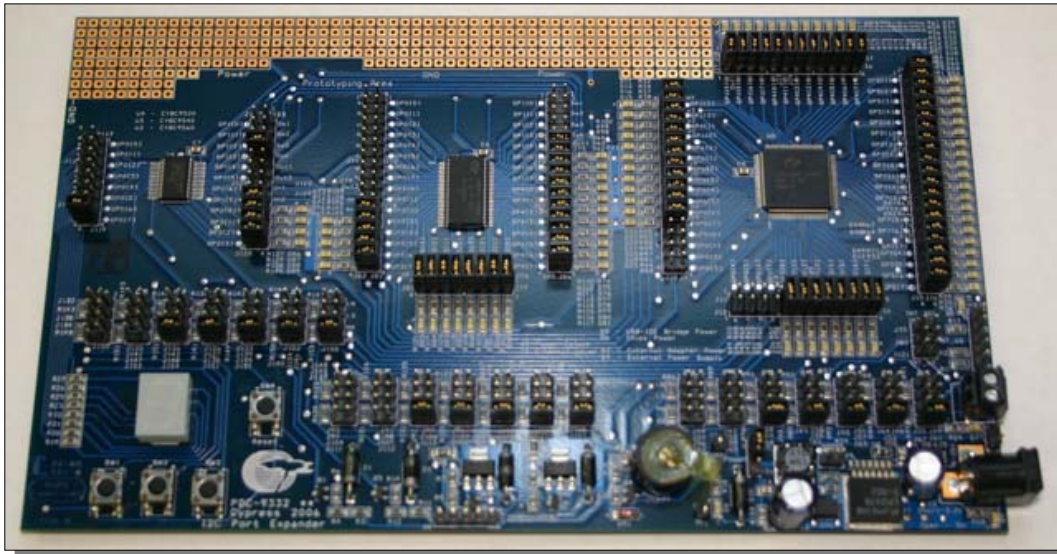
I2C Port Expander Evaluation Board
