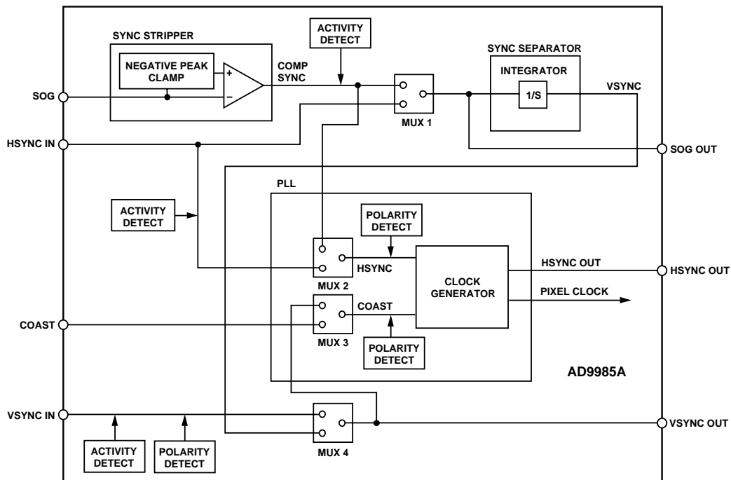
Figure 14. Sync Processing Block Diagram
