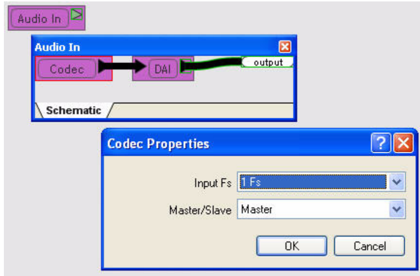
Figure 4-4. Audio In via 8 Channel ADC
