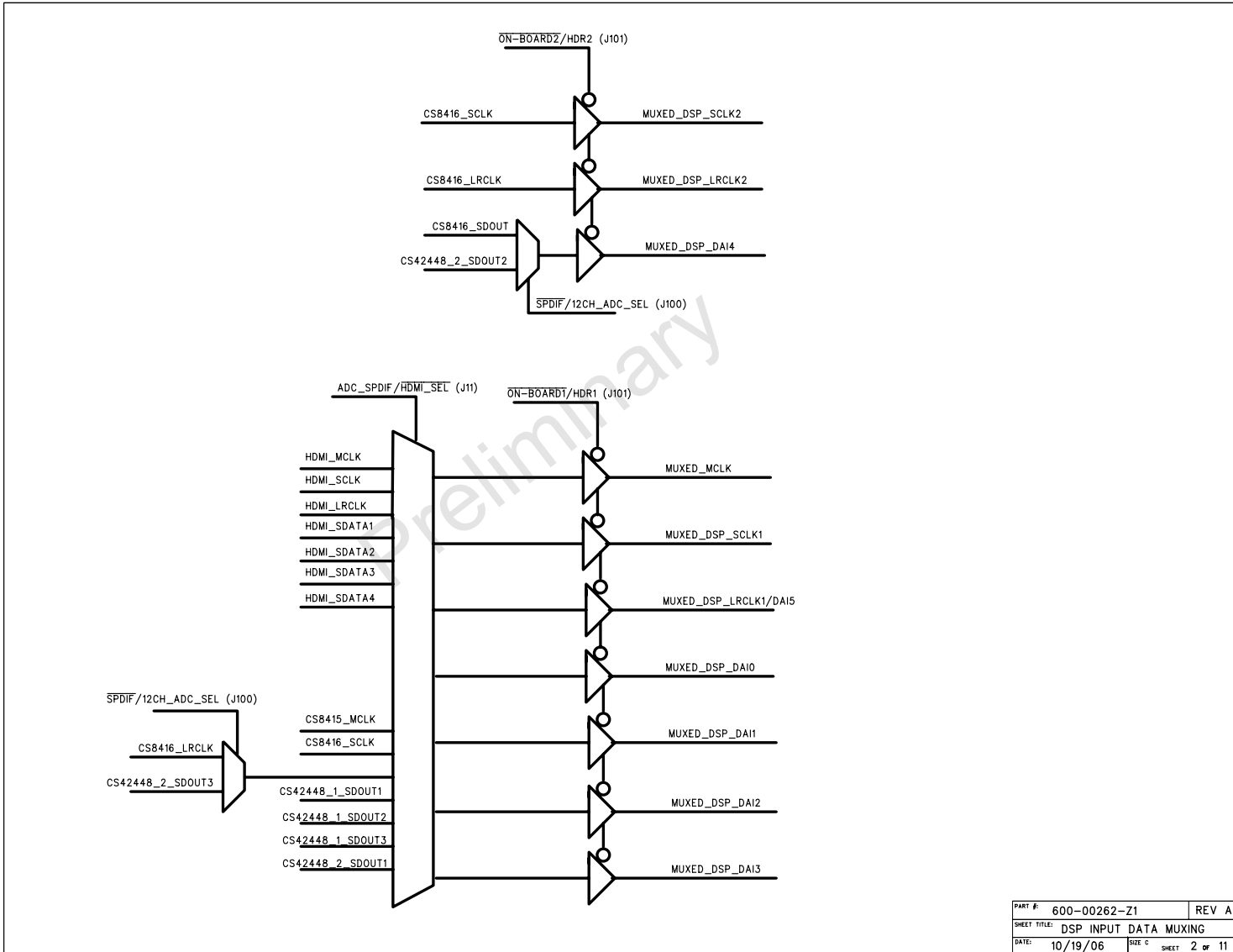
Figure A-2. DSP Input Data Multiplexing
