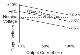
Tolerance Envelope Graph
