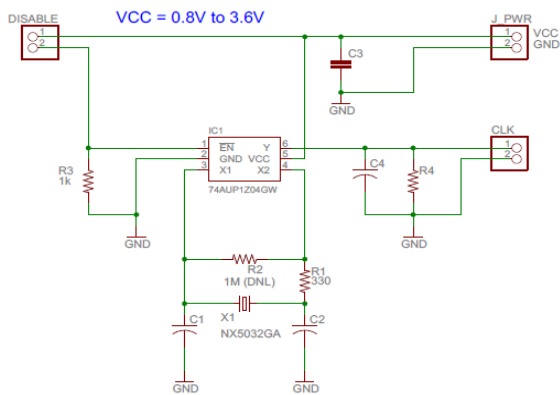
Demo board circuit schematics
