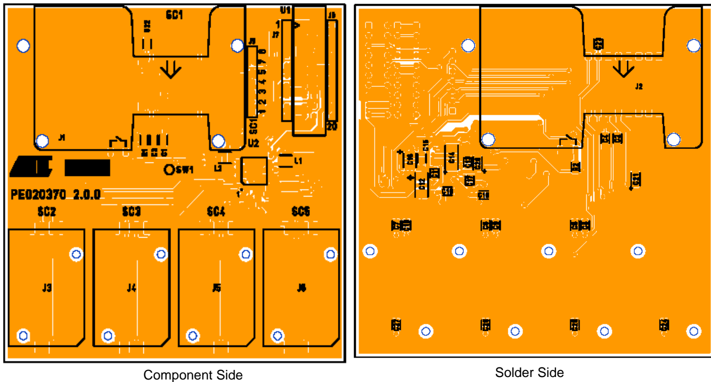
Figure 3-2. Component & Solder Sides
