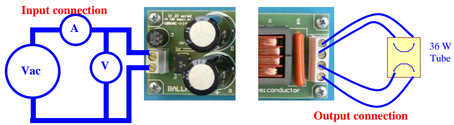
Figure 1: Ballast connection
