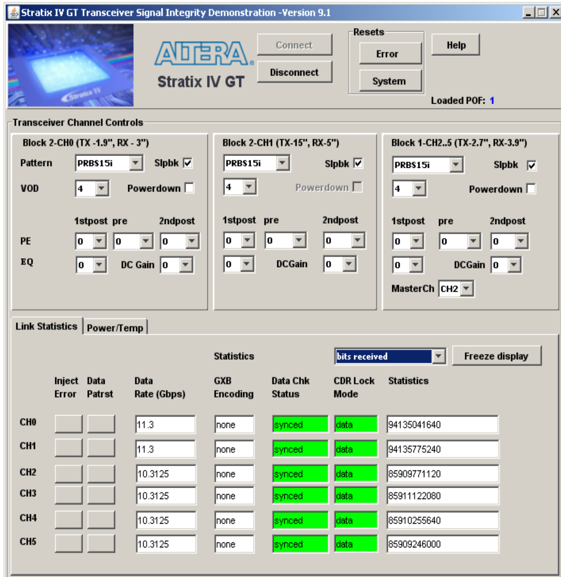
Figure 6-1. Demonstration Application Control Panel Window
