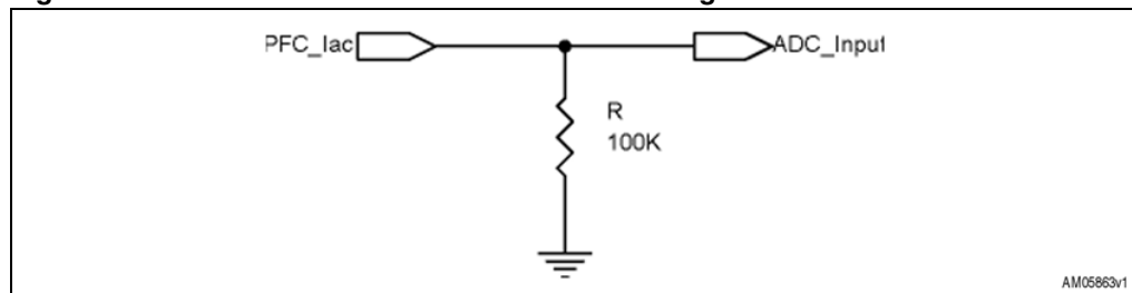
Figure 19. STEVAL-IHM022V1 - PFC current sensing section
