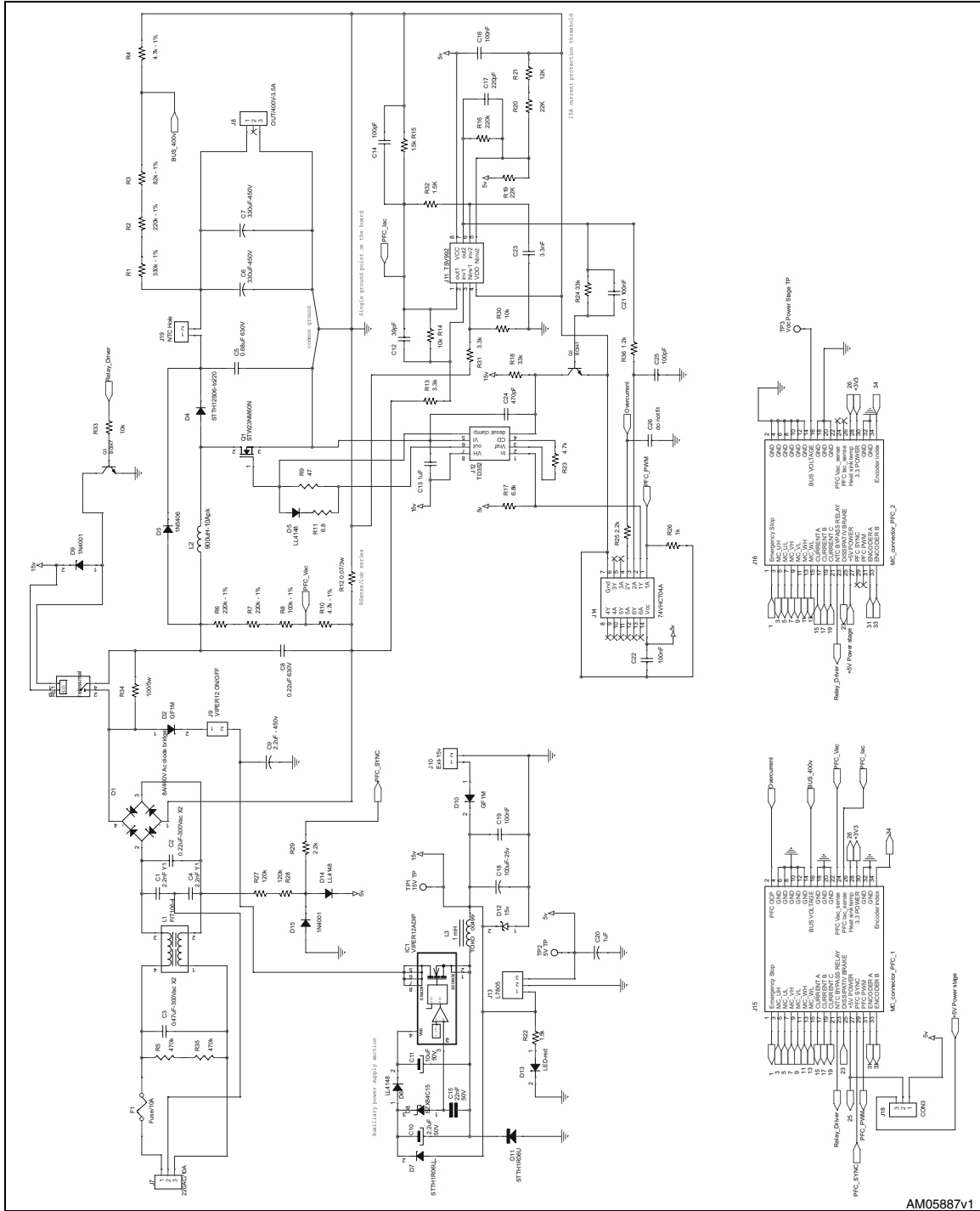
Figure 43. STEVAL-ISF00V1 schematic
