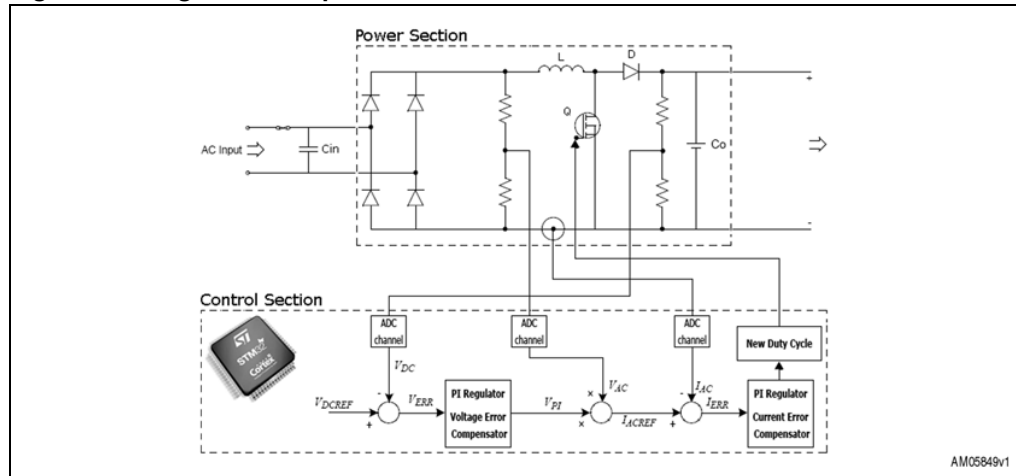
Figure 5. Digital PFC implementation scheme
