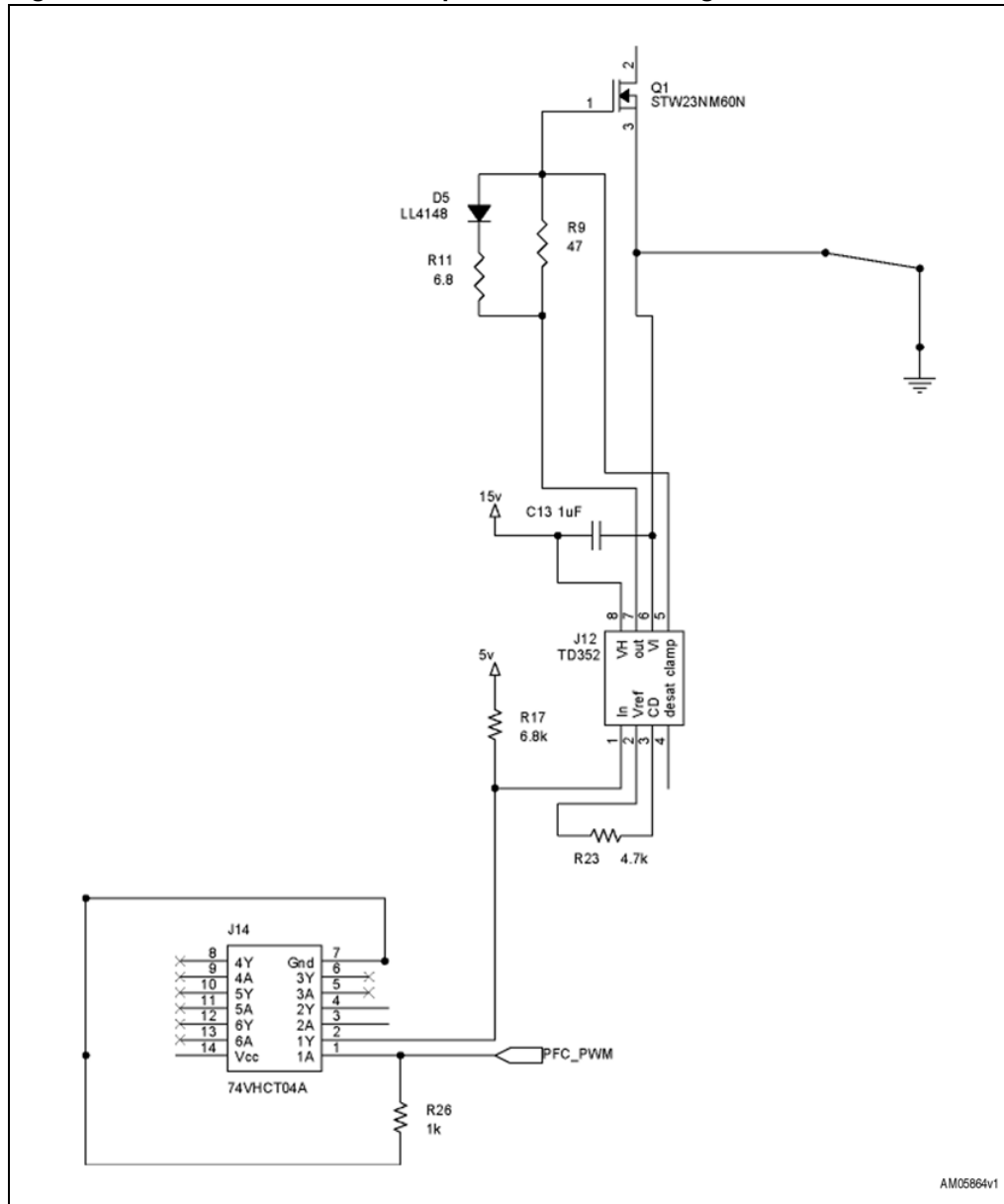
Figure 20. STEVAL-ISF002V1 - PFC power MOSFET driving section
