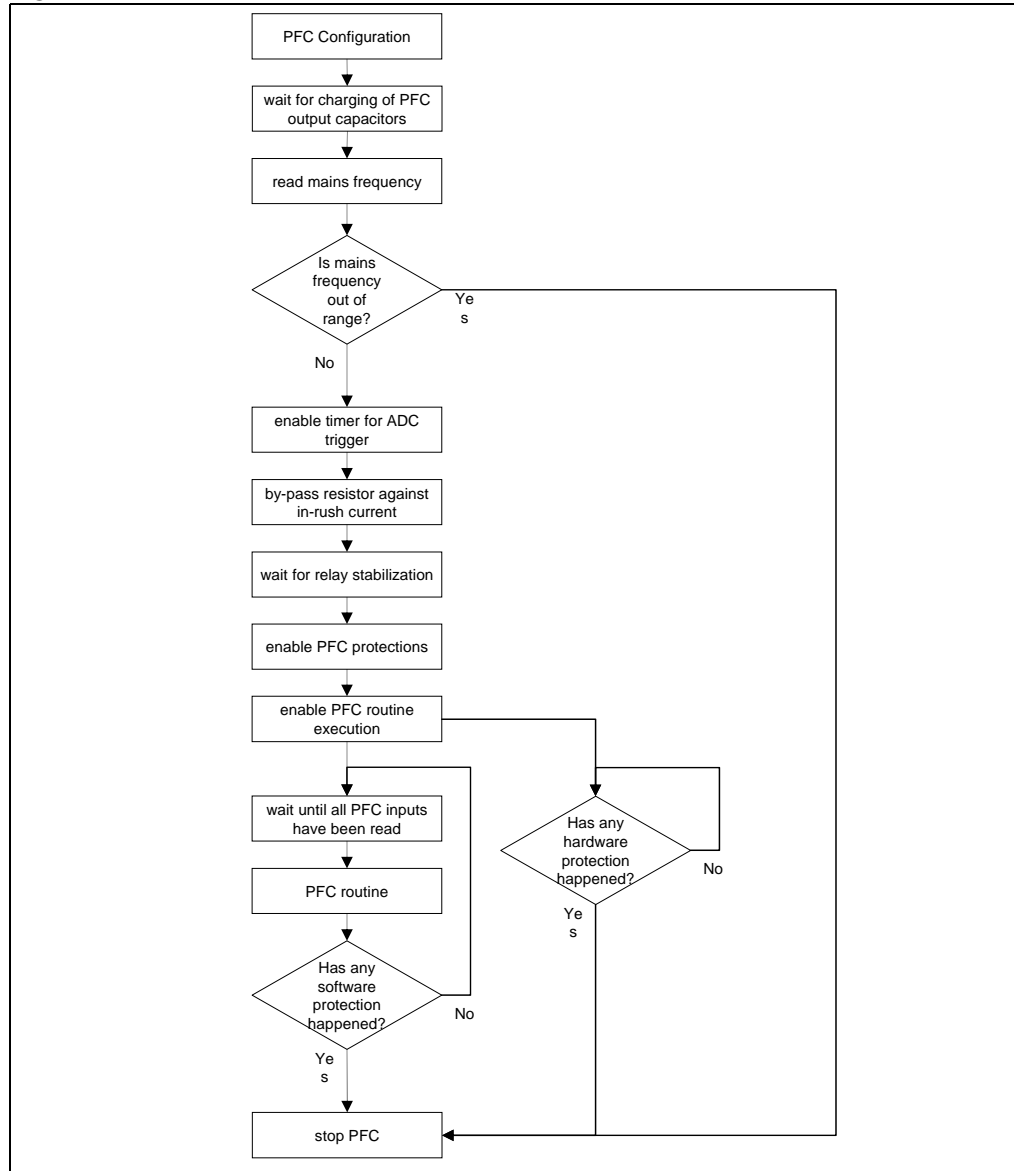
Figure 29. PFC firmware flowchart
