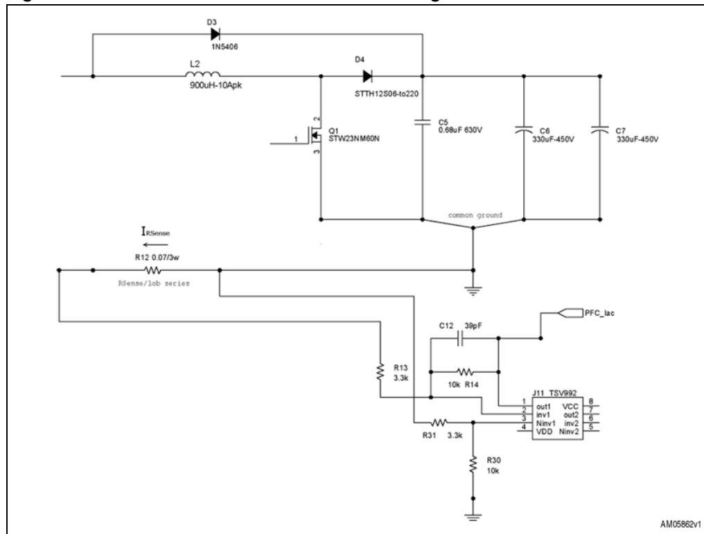
Figure 18. STEVAL-ISF002V1 - PFC current sensing section
