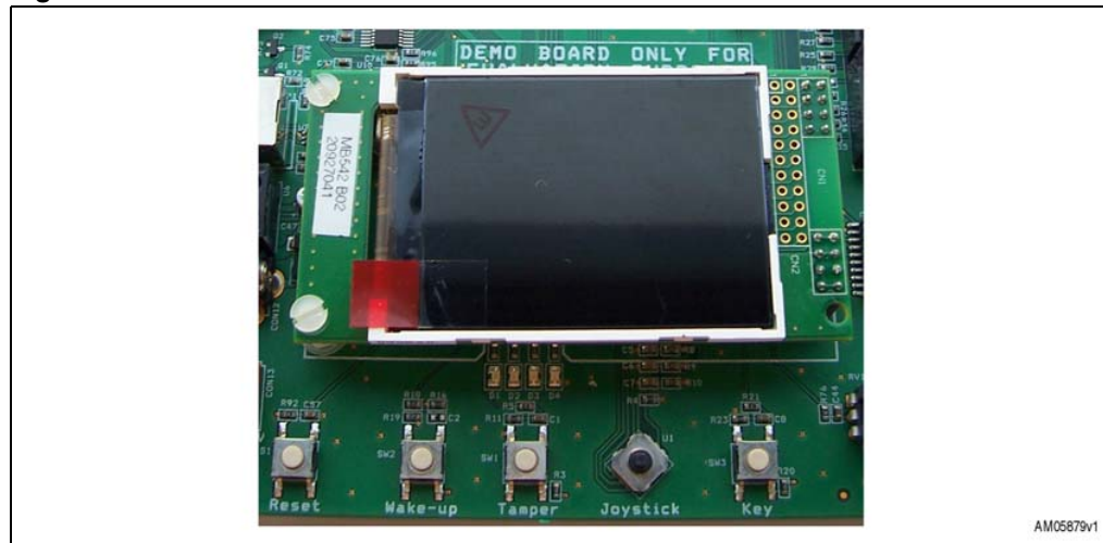
Figure 35. Hardware elements of the control board
