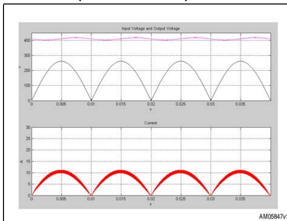
Figure 3. AC to DC boost converter signals with CCM PFC - output VDC, input Vac and inductor current (time scale = 5 ms)
