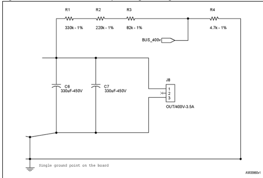
Figure 17. STEVAL-IHM022V1 - output voltage sensing section
