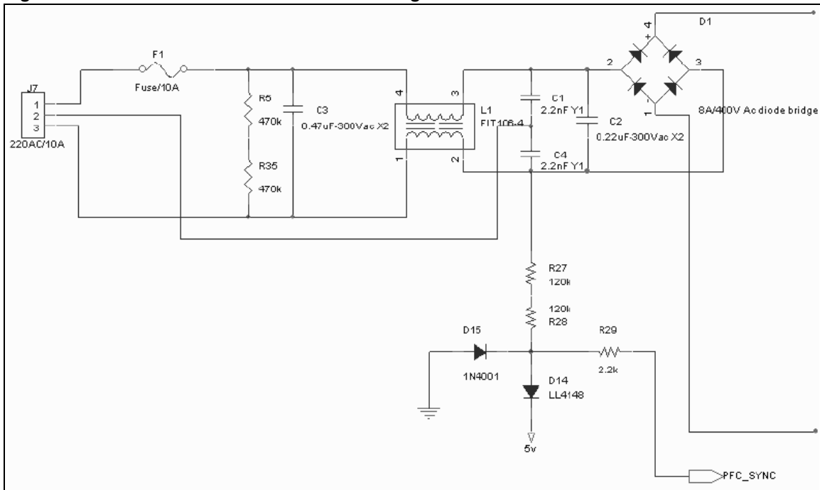
Figure 22. STEVAL-ISF002V1 - vin zero crossing detection section
