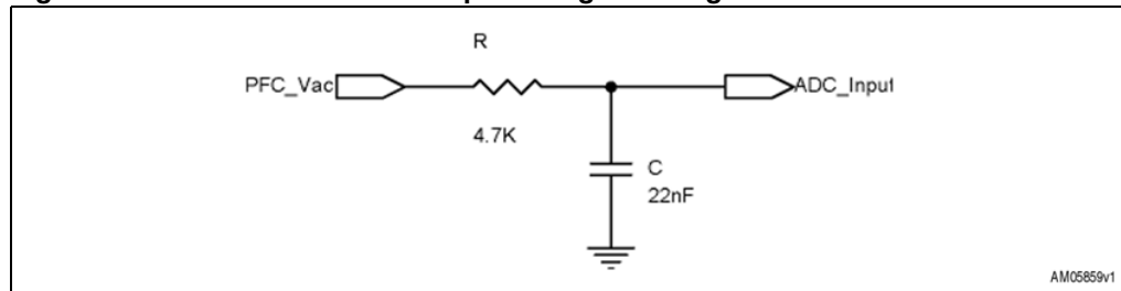
Figure 15. STEVAL-IHM022V1 - input voltage sensing section
