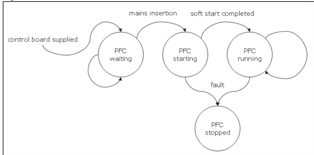
Figure 27. PFC states
