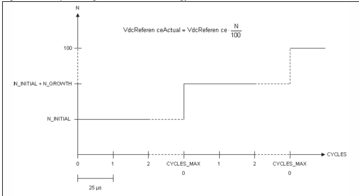
Figure 26. Output voltage soft-start methodology
