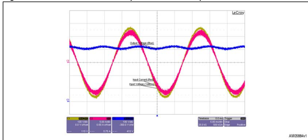
Figure 40. 185 Vrms at 50 Hz as input - 1400 W as output load
