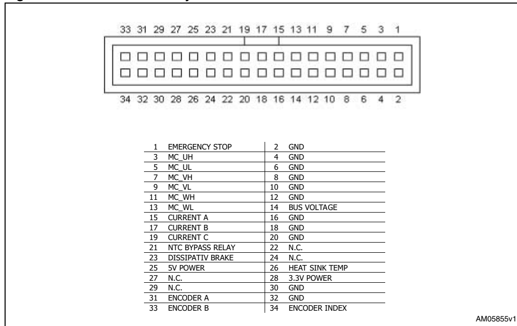
Figure 11. MC connector only
