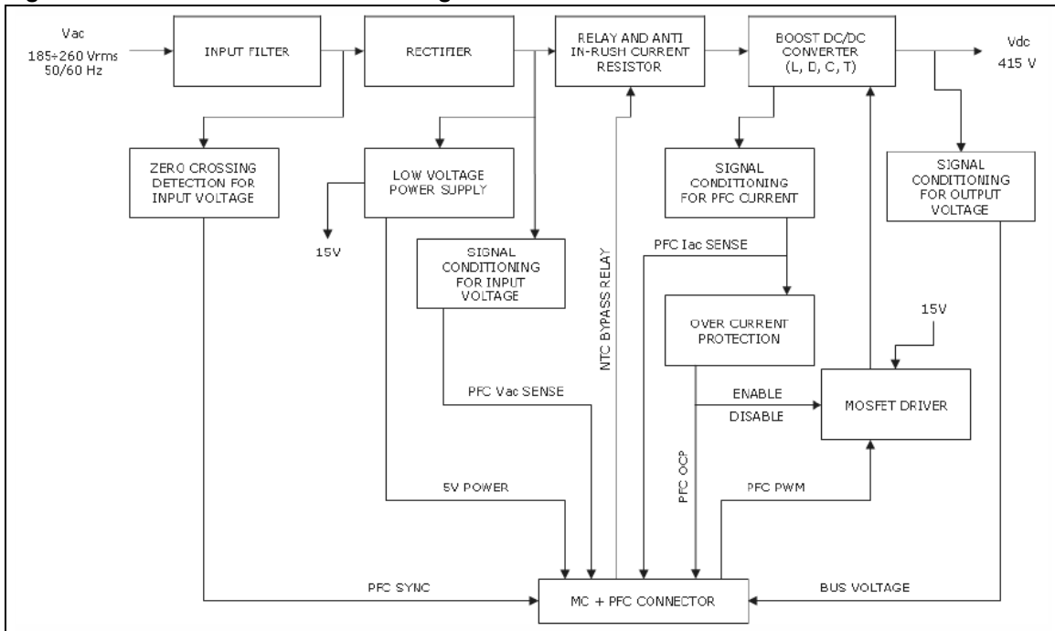
Figure 12. STEVAL-ISF001V1 block diagram
