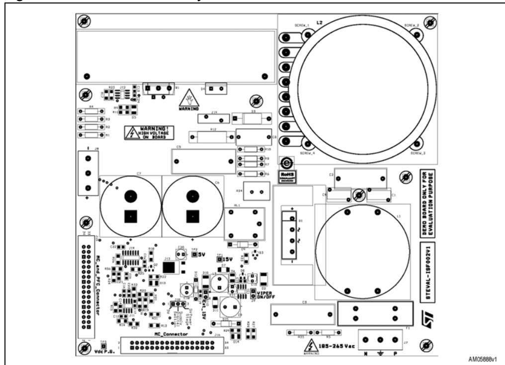
Figure 44. STEVAL-ISF002V1 layout
