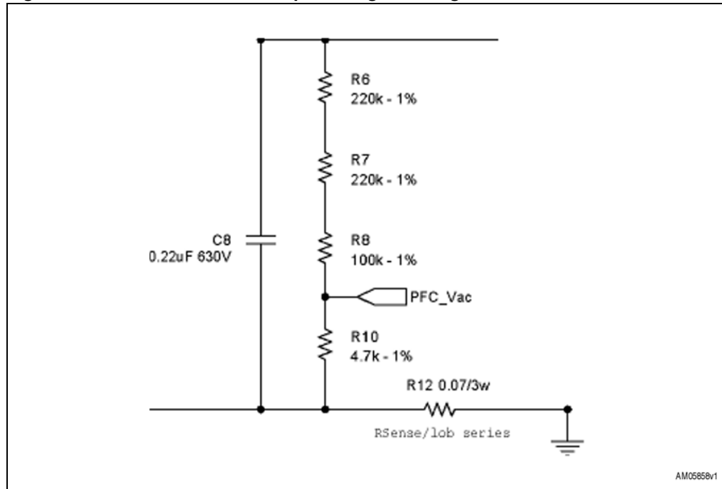
Figure 15. STEVAL-IHM022V1 - input voltage sensing section
