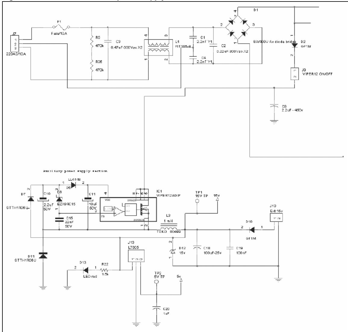
Figure 13. STEVAL-ISF002V1 - power supply section
