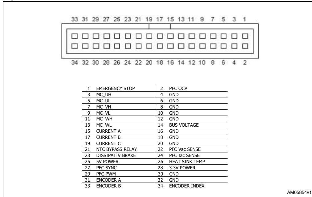
Figure 10. MC + PFC connector
