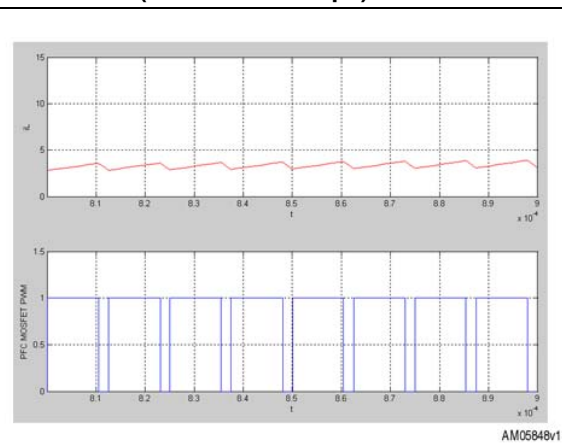
Figure 4. AC to DC boost converter signals with CCM PFC - inductor current and power MOSFET gate command (time scale = 10 μs)
