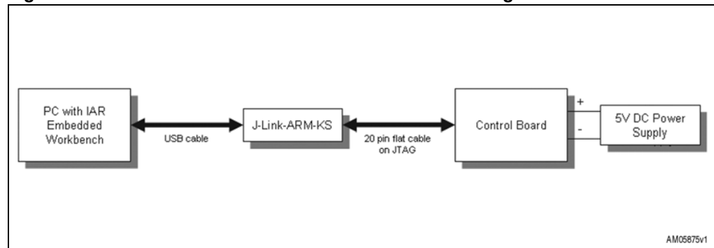
Figure 31. Hardware connections for firmware downloading
