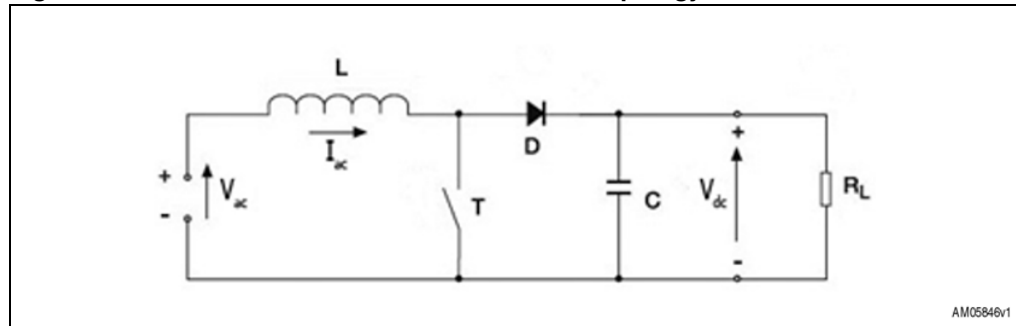
Figure 2. Scheme of AC to DC boost converter topology
