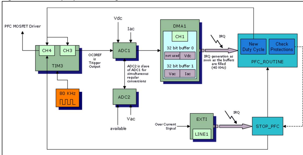
Figure 28. Use of peripherals for digital PFC
