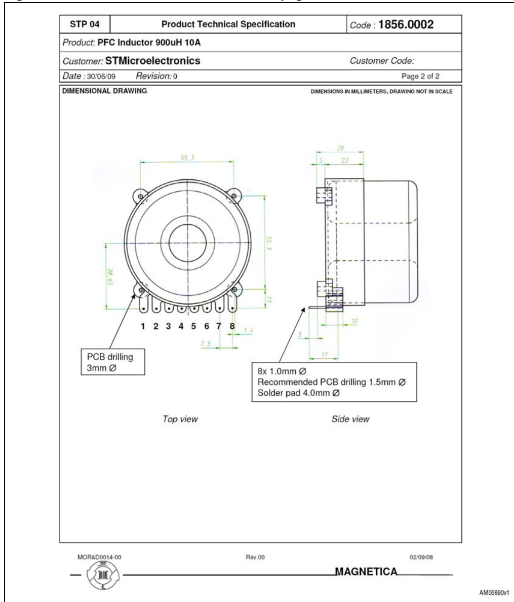
Figure 46. Technical sheet of PFC inductor - page 2 of 2
