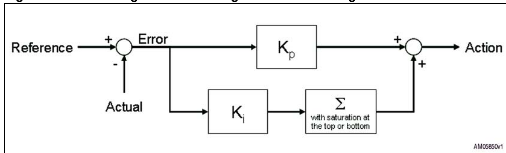
Figure 6. Block diagram of the voltage and current PI regulator
