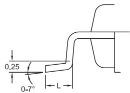
Figure 58. 32-Pin Low Quad Flat Package
