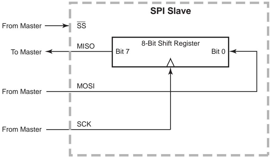
Figure 24. SPI Configured as a Slave
