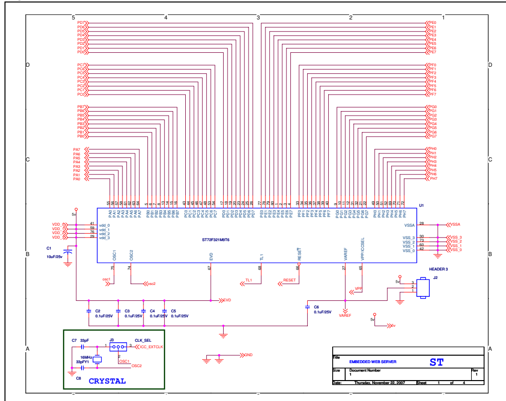
Figure 1. Microcontroller
