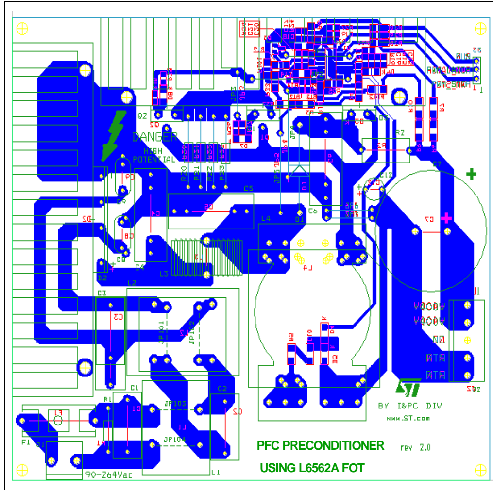
Figure 2. PCB layout(a)
