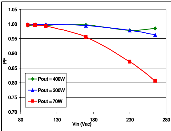
Figure 7. Power factor vs. V_{in} and load
