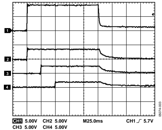
Figure 2. Sequenced Waveforms
