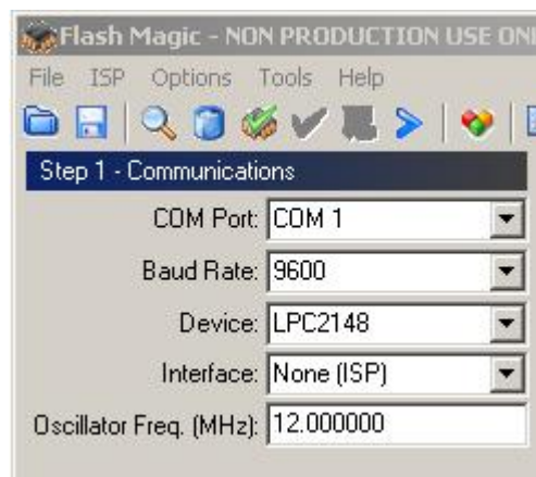
Fig 11. Settings for connecting with serial ISP
