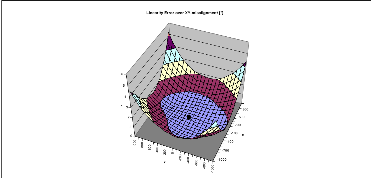
Figure 25 Example of Linearity Error over XY Misalignment
