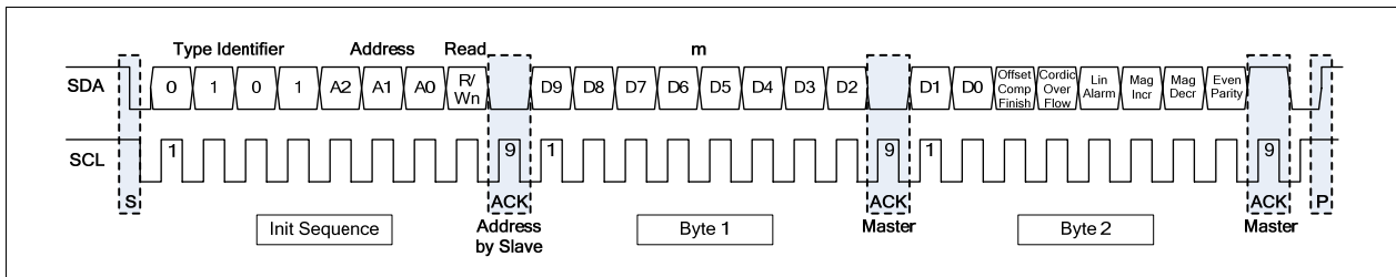
Figure 7 16-bit Serial Read / Write Timing
