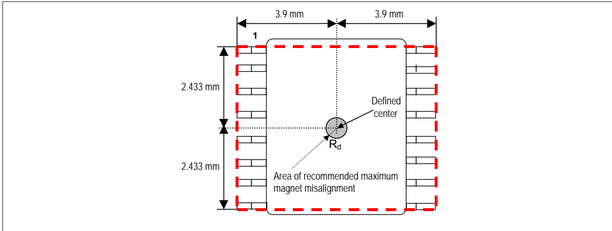
Figure 22 Defined IC Center and Magnet Displacement Radius
