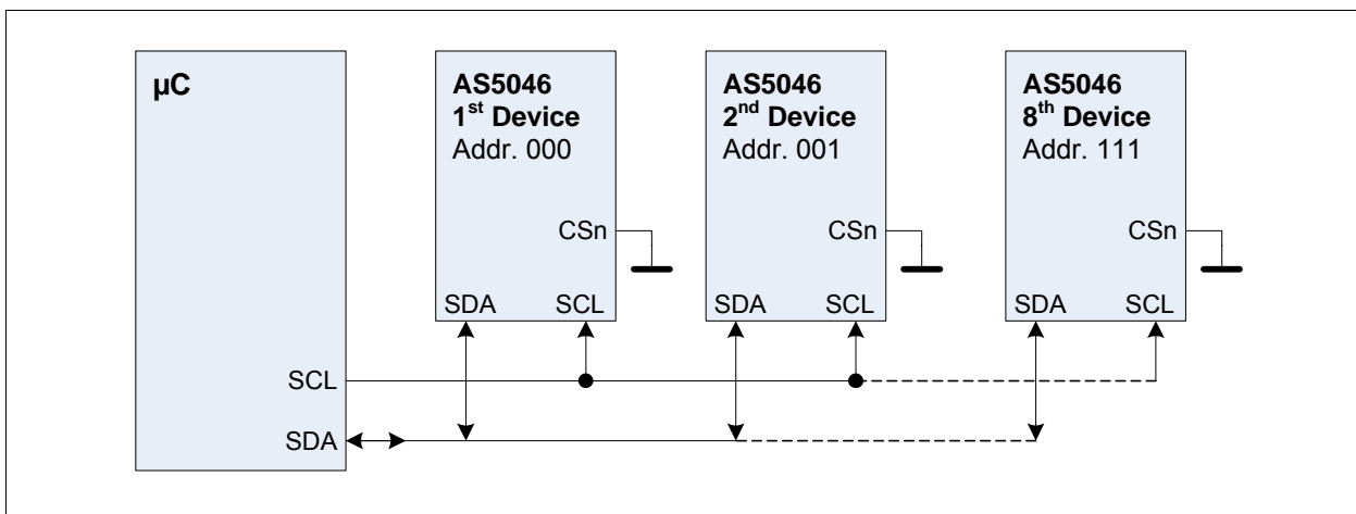
Figure 10 Parallel Connection of up to 8 Devices
