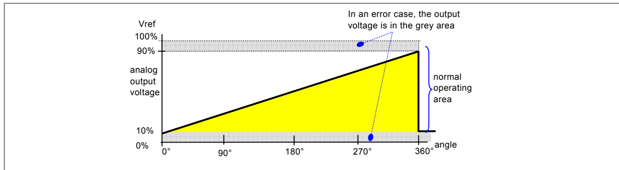
Figure 12 Diagnostic Output Mode
