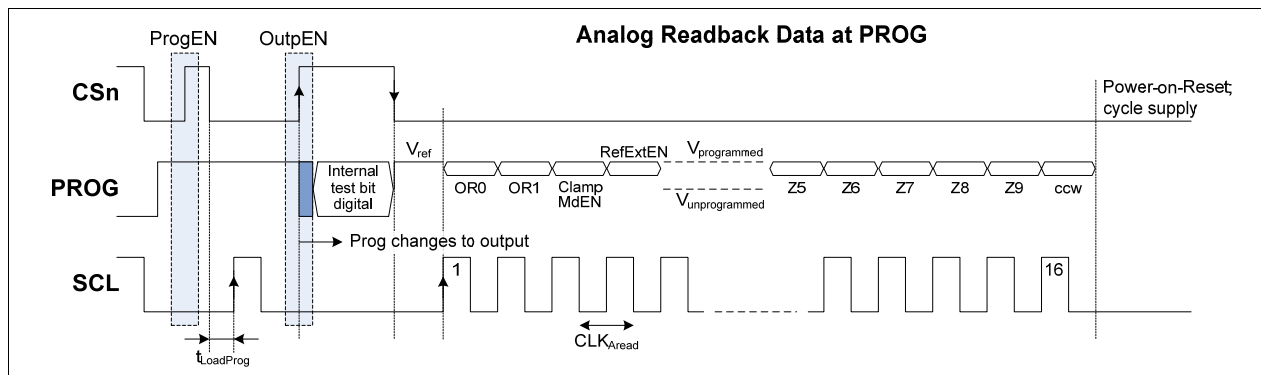
Figure 18 Analog OTP Register Read
