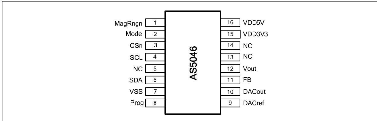
Figure 3 AS5046 Pin Configuration SSOP16
