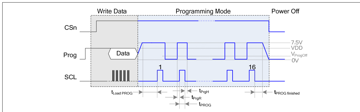
Figure 14 Complete OTP Programming Sequence
