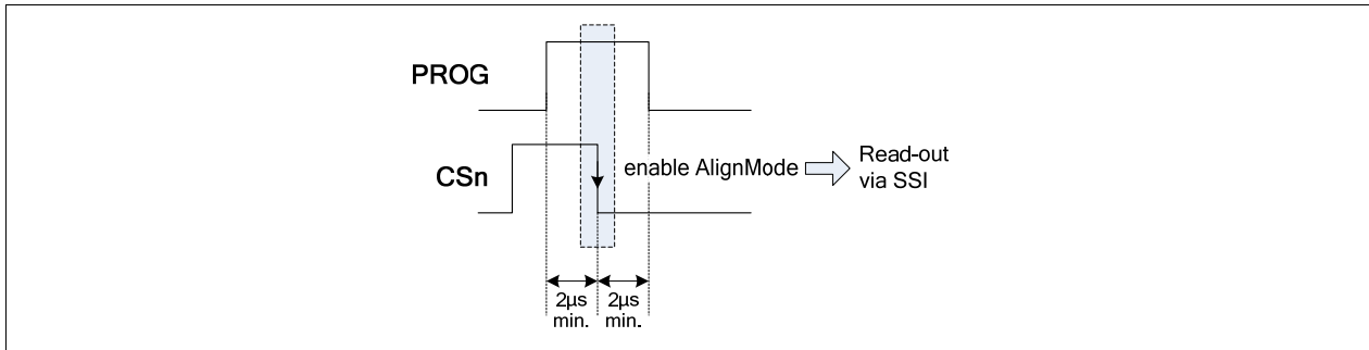
Figure 19 Enabling the Alignment Mode
