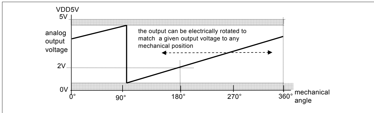
Figure 16 Zero Position Programming (shown for 360° mode)
