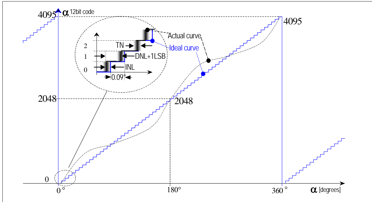
Figure 4 Integral and Differential Non-Linearity (exaggerated curve)
