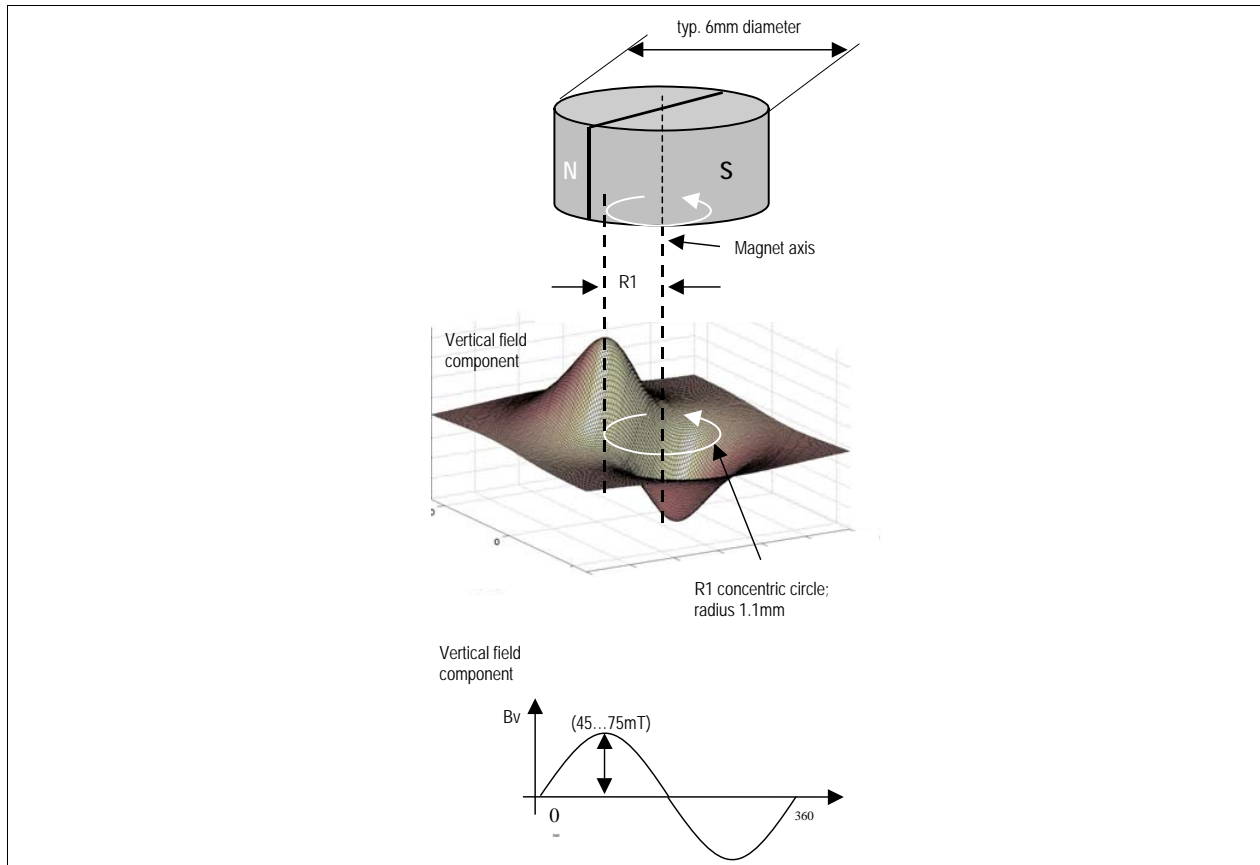
Figure 21 Typical Magnet and Magnetic Field Distribution
