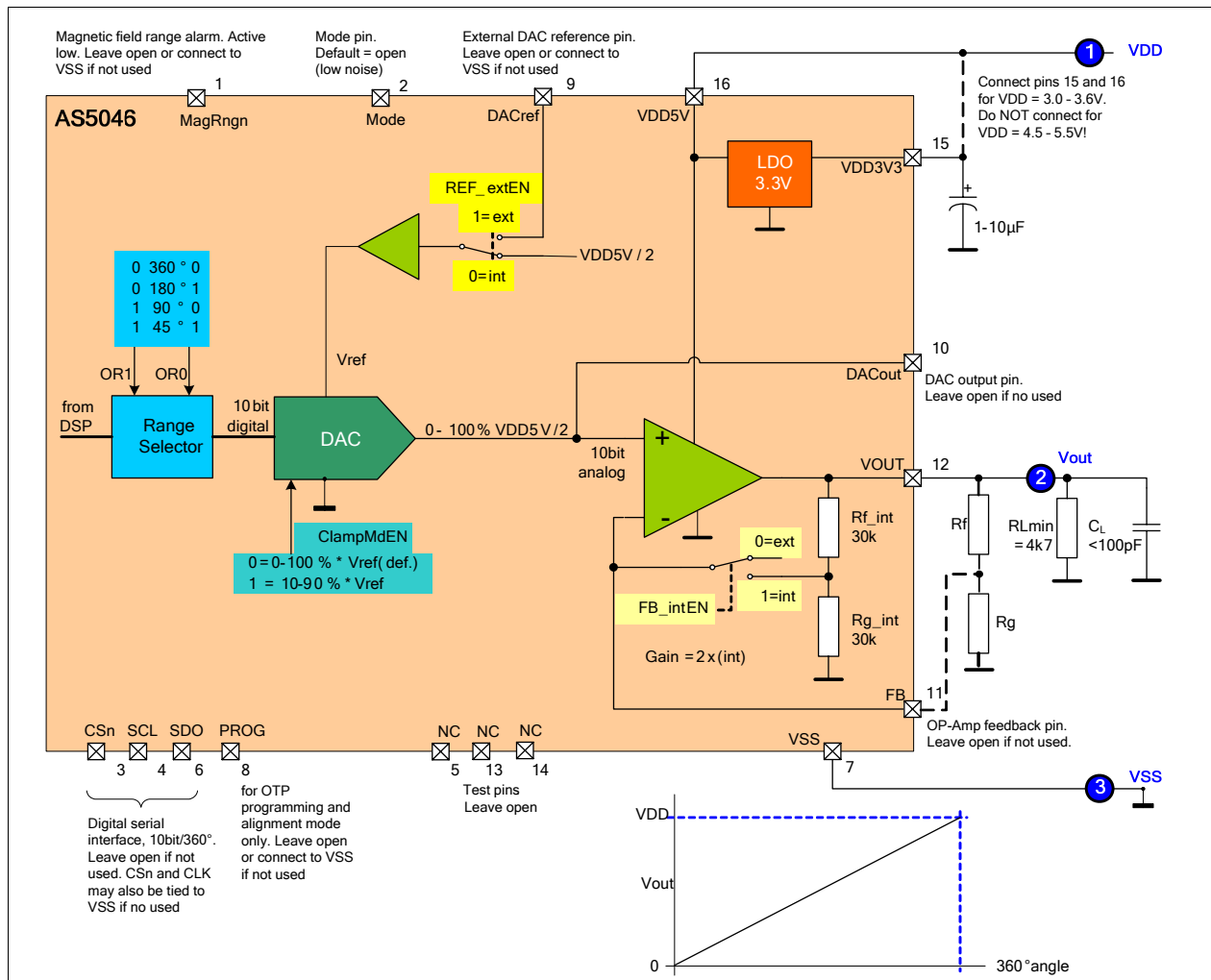
Figure 17 Analog Output Block Diagram
