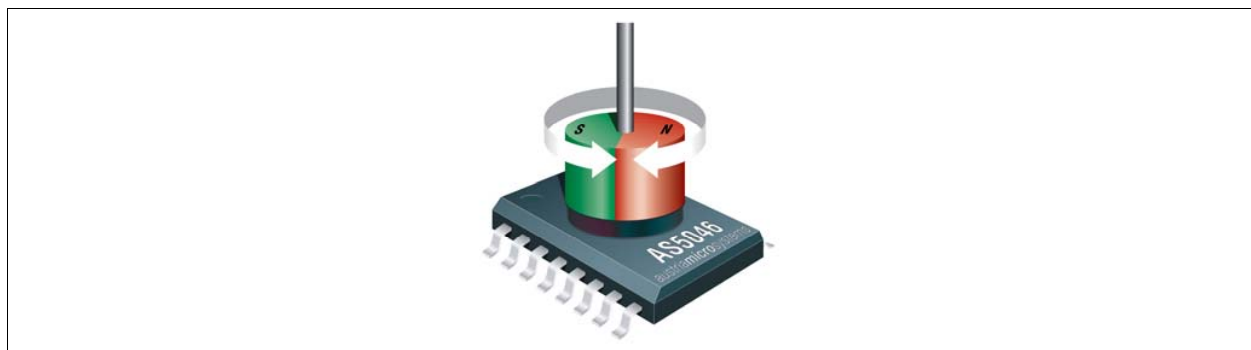
Figure 1 Typical Arrangement of AS5046 and Magnet
