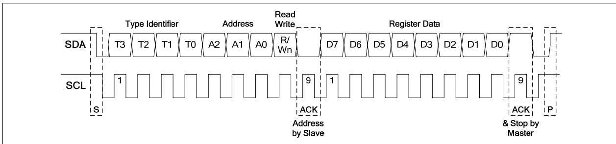
Figure 6 8-bit Serial Read / Write Timing
