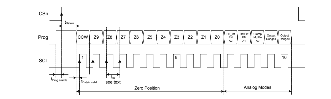
Figure 14 Complete OTP Programming Sequence
