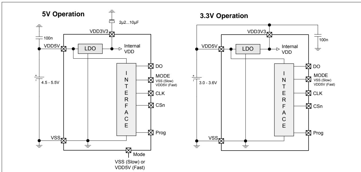
Figure 5 Connections for 5V / 3.3V Supply Voltages
