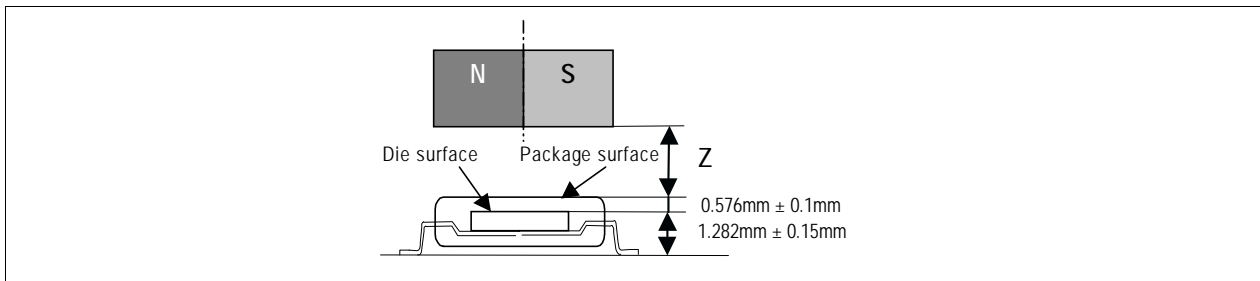
Figure 23 Vertical Placement of the Magnet
