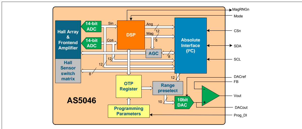
Figure 2 AS5046 Block Diagram
