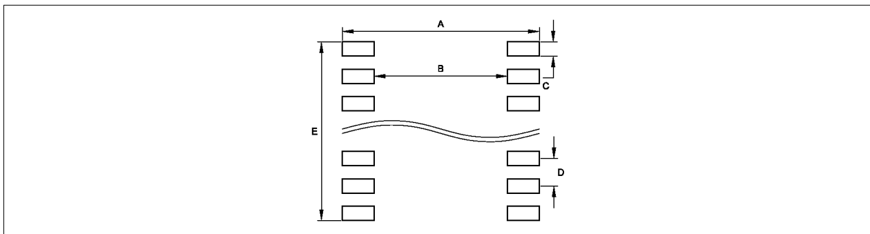
Figure 28 Recommended PCB Footprint
