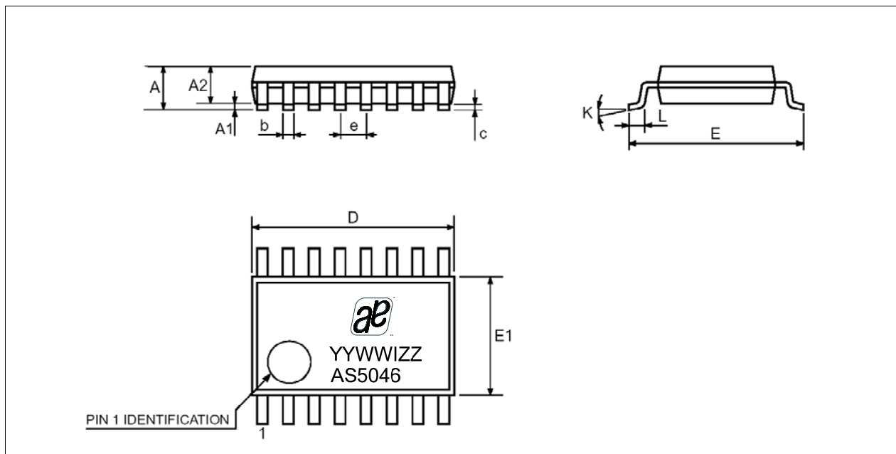
Figure 27 Package Drawings and Marking
