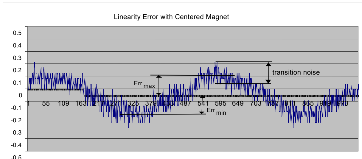
Figure 26 Example of Linearity Error over 360°
