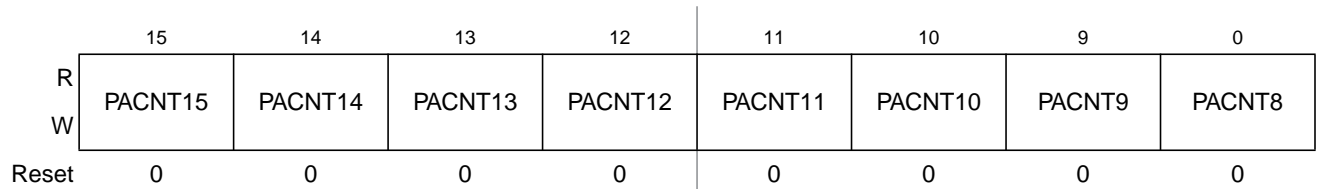
Figure 16-26. Pulse Accumulator Count Register High (PACNTH)
