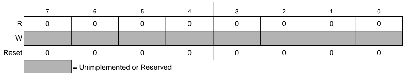
Figure 2-13. PIM Reserved Register
