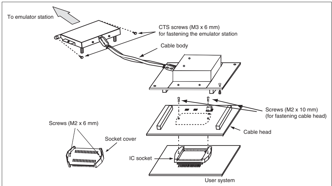
Figure 1 HS36902ECF61H User System Interface Cable
