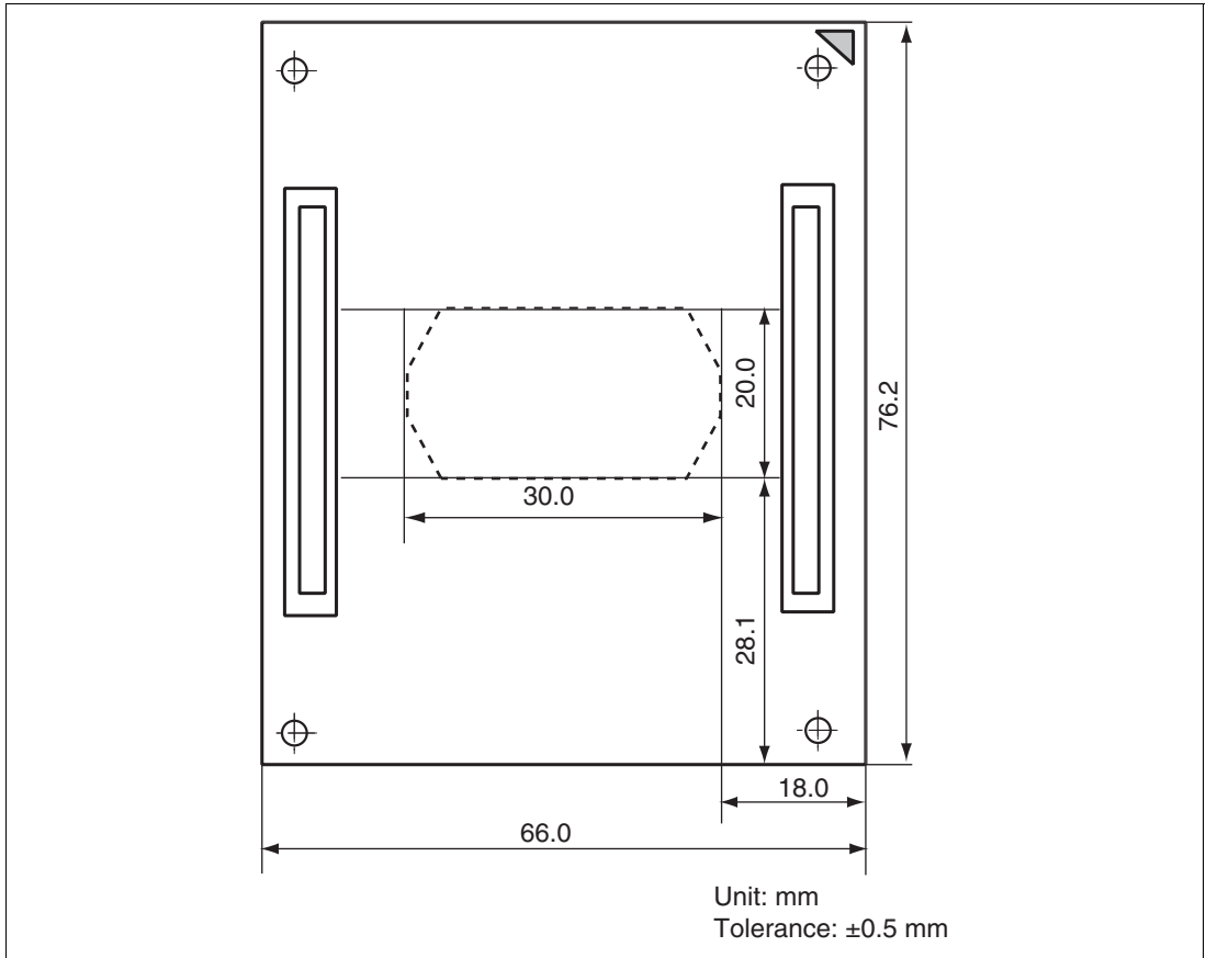
Figure 7 Dimensions for User System Interface Cable Head
