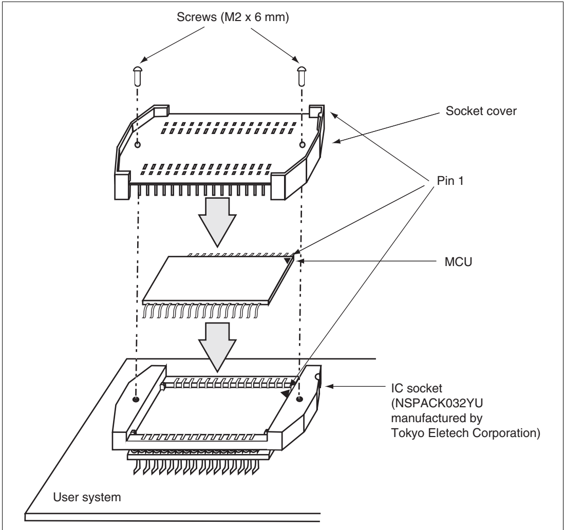
Figure 9 Installing MCU to User System
