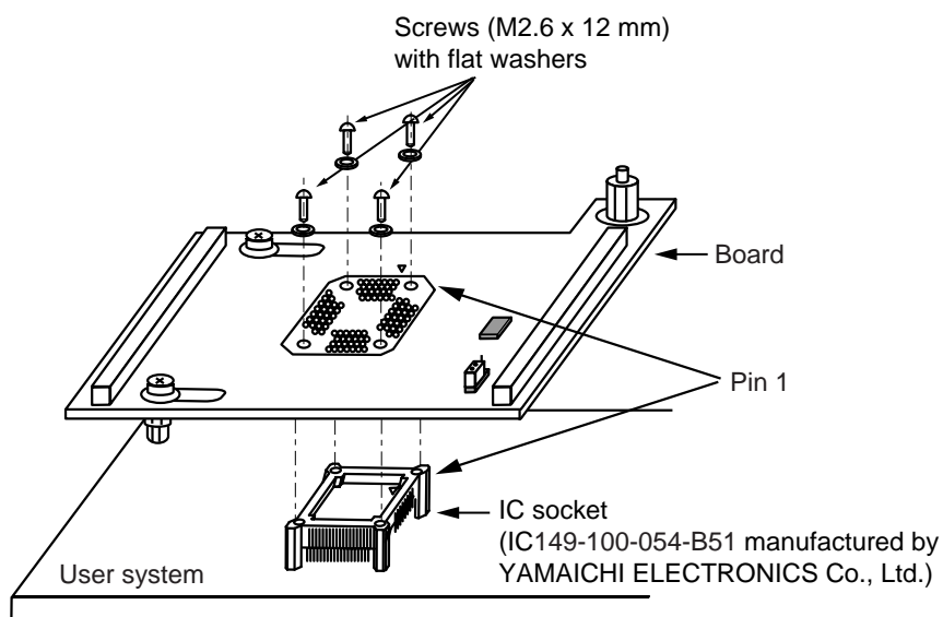
Figure 2 Connecting User System Interface Board to User System
