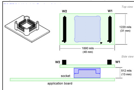
Figure 2. TQFP64 device adapter (DB543)
