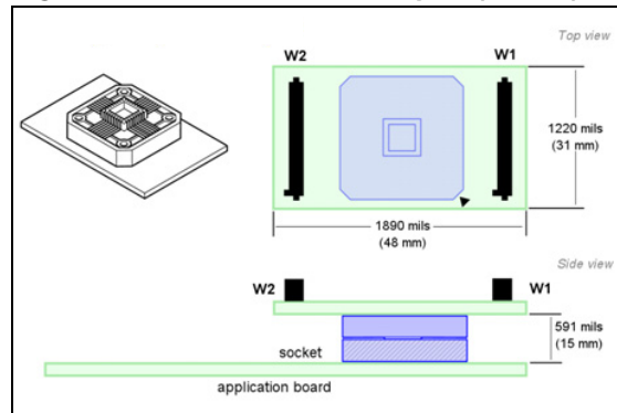
Figure 2. TQFP44 device adapter (DB544)
