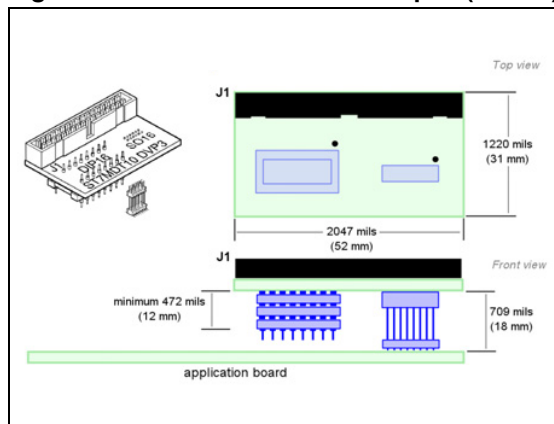
Figure 1. DIP16/SO16 device adapter (DB587)
