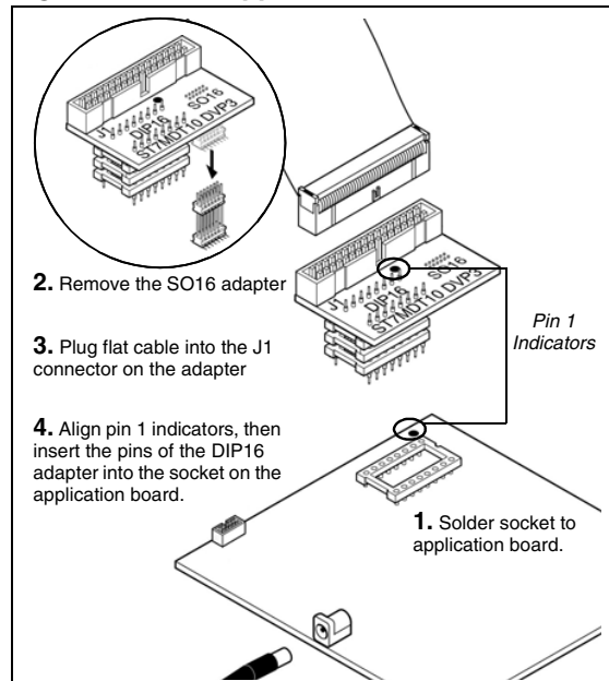
Figure 2. DIP16 application board connection
