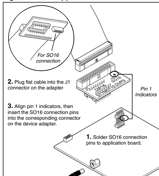
Figure 3. SO16 application board connection
