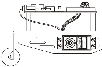
Servo head is mounted toward tail wheel
