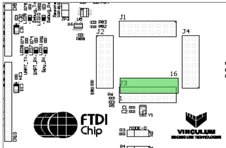
Figure 5.24 VNC2 Daughterboard Connector J3
