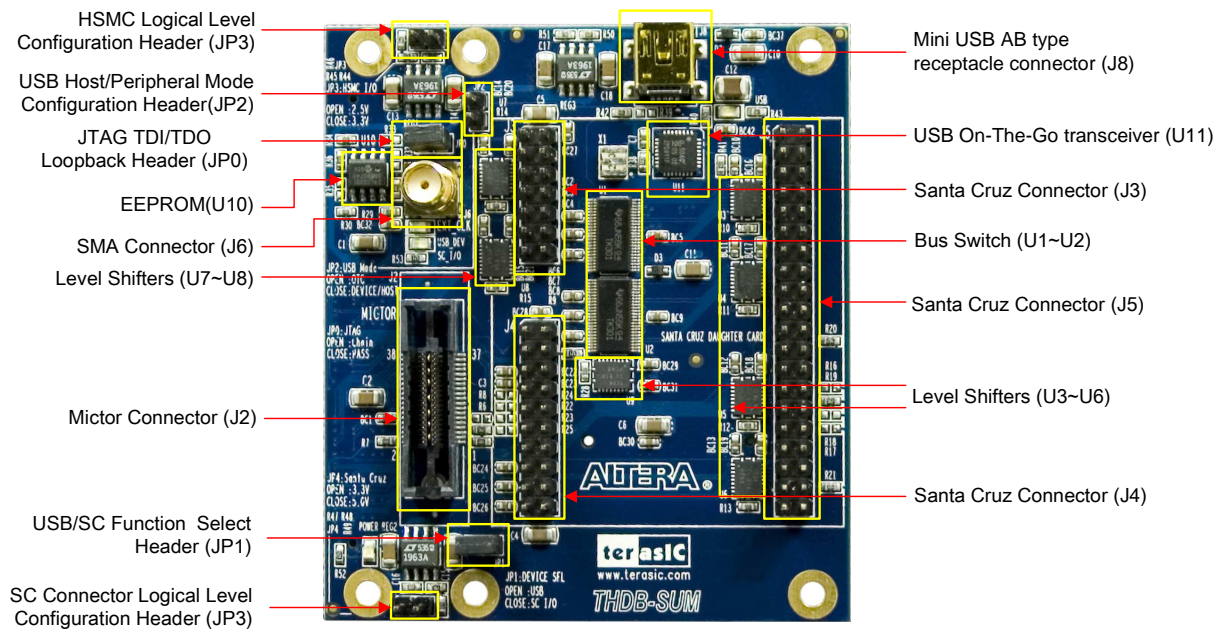
Figure 2.1. The THDB-SUM PCB and component diagram
