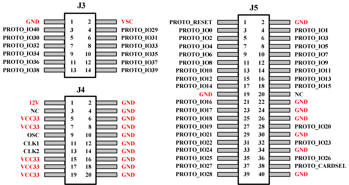
Figure 3.7 Santa Cruz connector pin-outs
