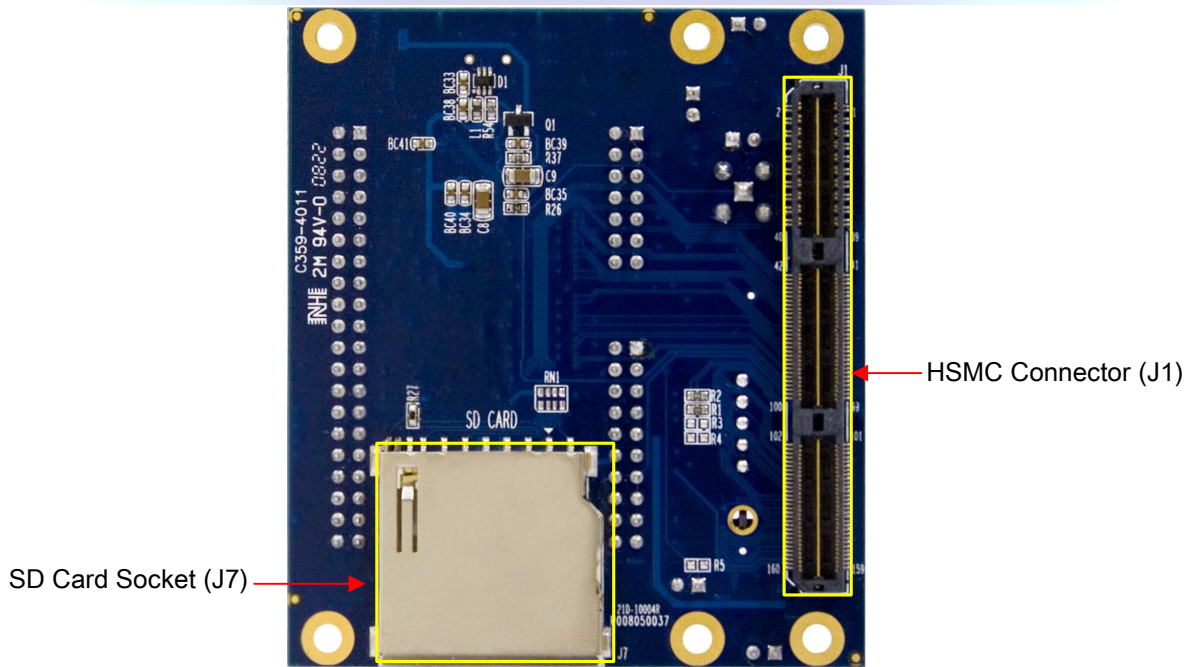
Figure 2.2. The THDB-SUM Back side – HSMC connector view
