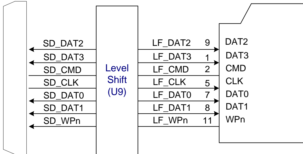
Figure 3.12 The block diagram of the SD Card socket and HSMC connector
