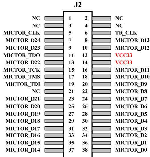
Figure 3.9 Mictor connector pin-outs
