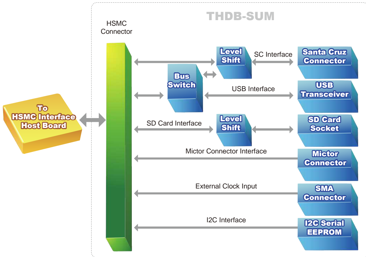
Figure 2.3. The block diagram of the THDB-SUM board
