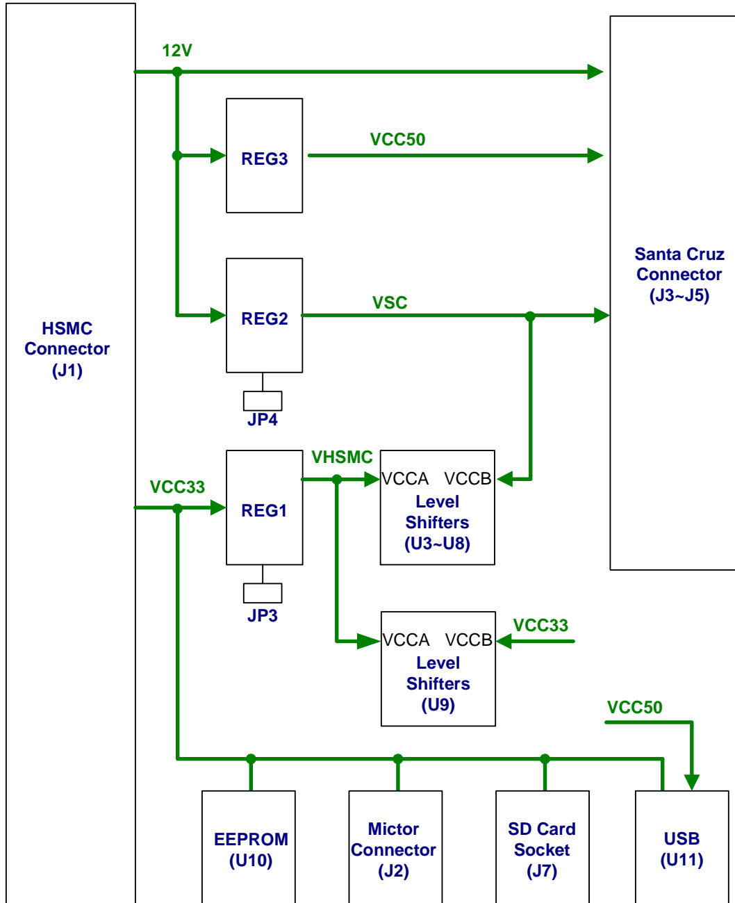
Figure 3.14. THDB-SUM board power distribution diagram.
