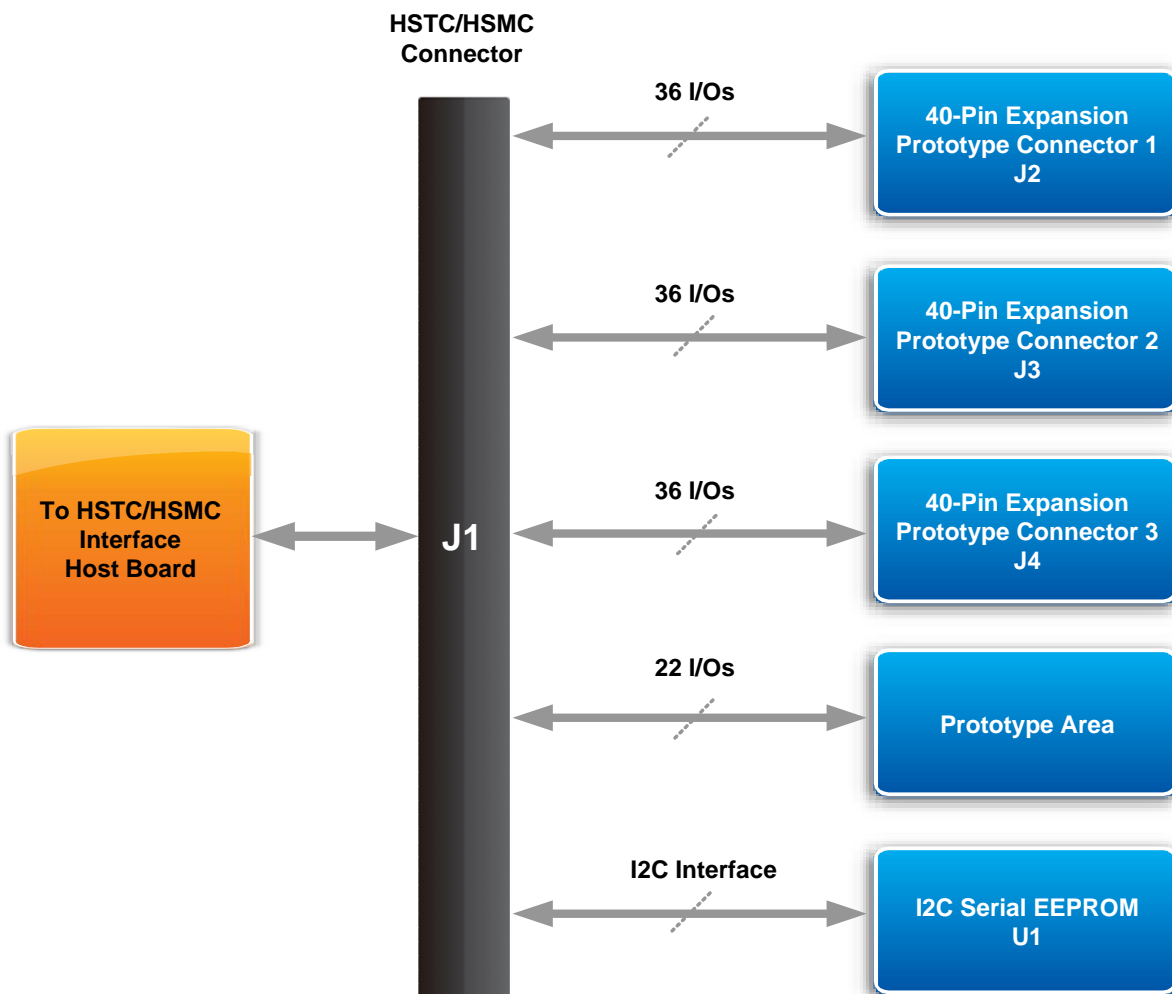
Figure 2.4. The block diagram of the THDB-HTG board
