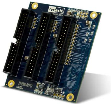
Figure 1.1. The picture of a THDB-HTG board
