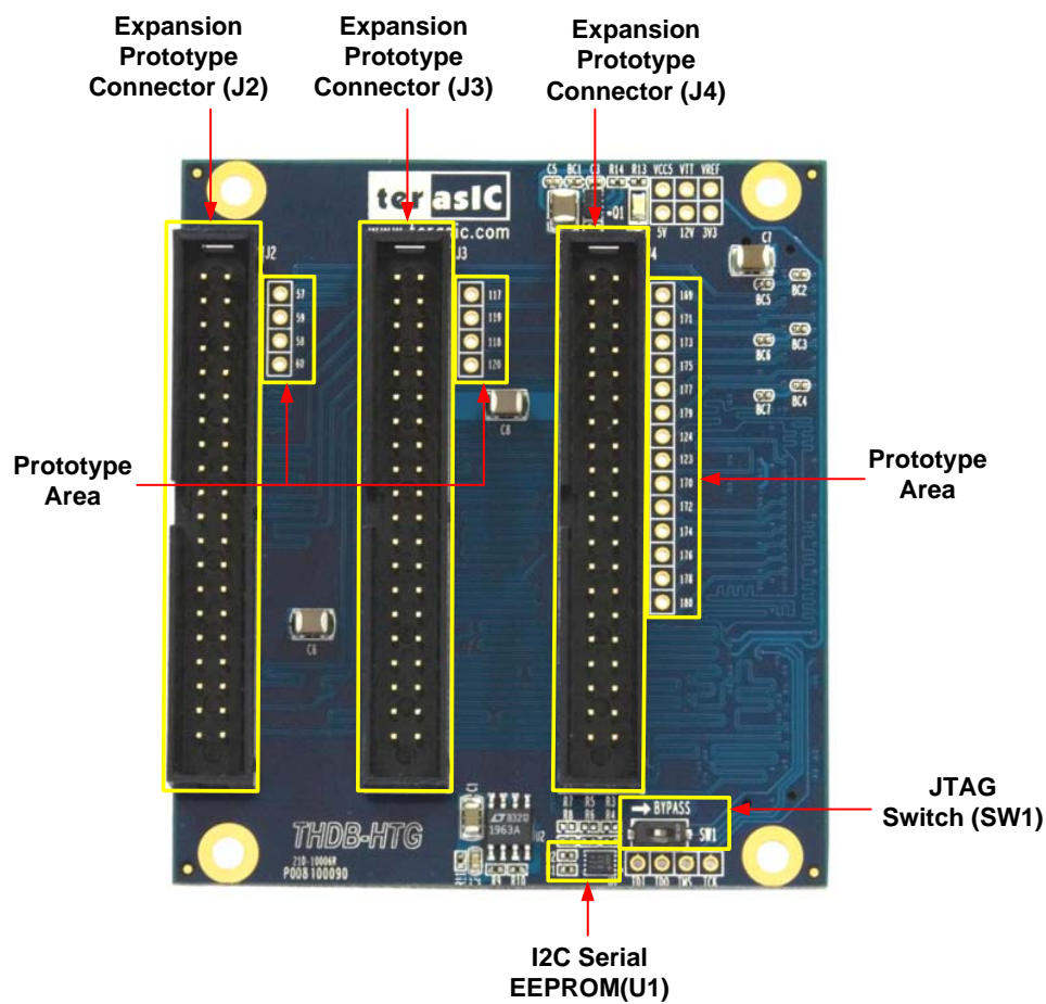
Figure 2.1 Top view of the TDRB-HTG board
