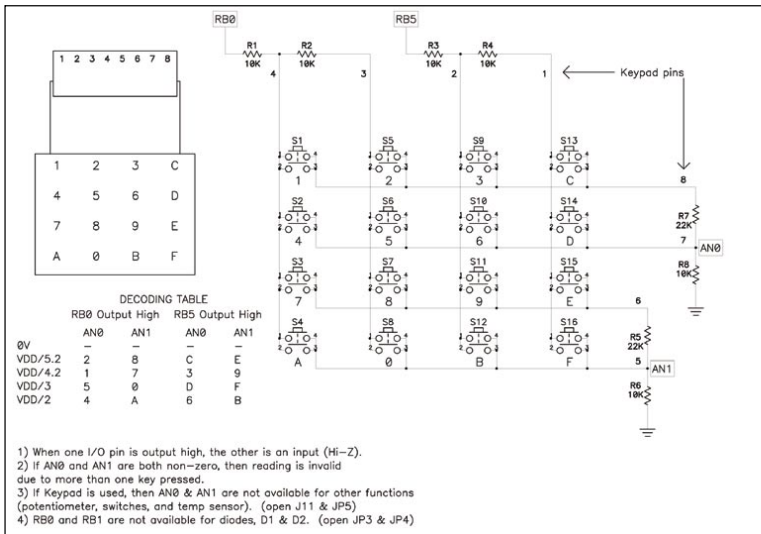
Figure 4-1: Keypad Hook-up Schematic
