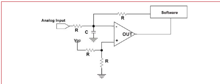
Figure 1: Delta-Sigma Converter Using a Standard Microcontroller
