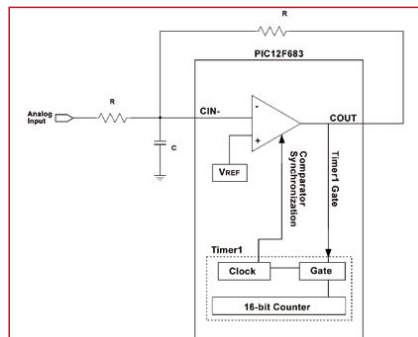
Figure 2: Delta-Sigma Converter Using the PIC12F683
