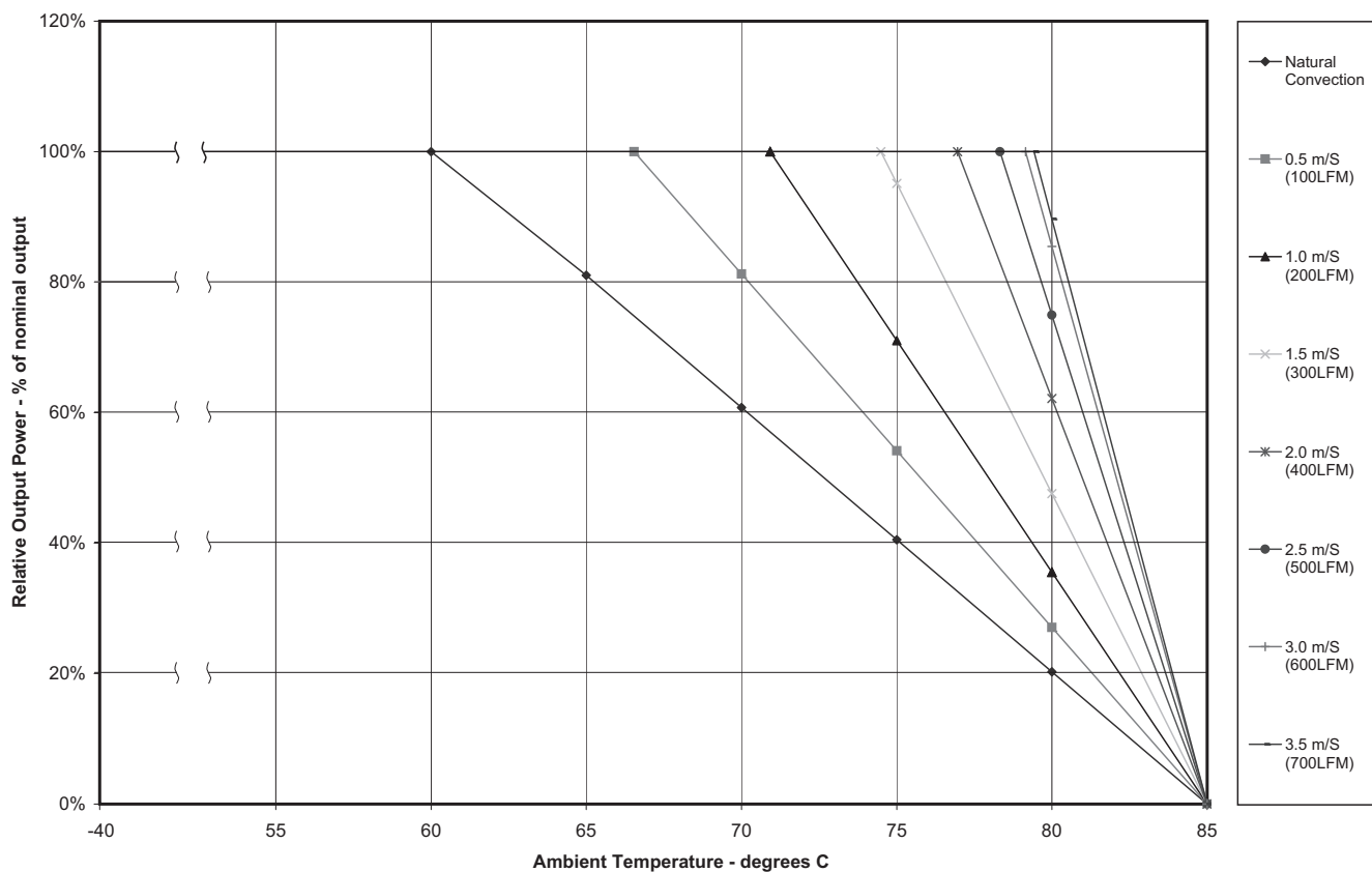
FIGURE 1. OUTPUT DERATING
