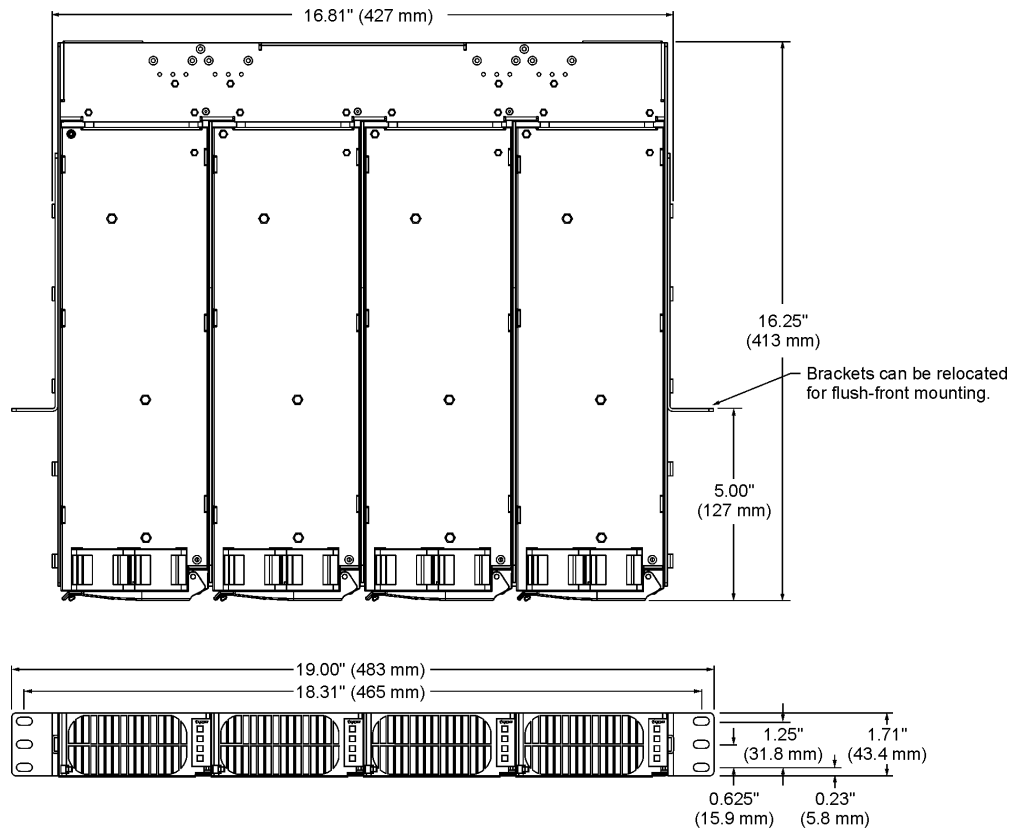
Package Outline
