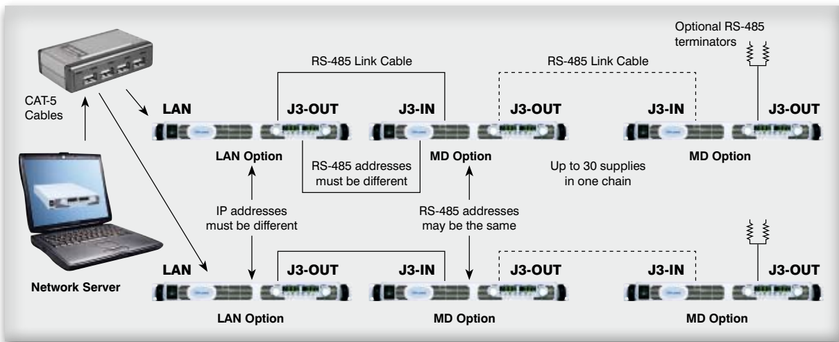
Configuring a Multi-drop system of supplies
