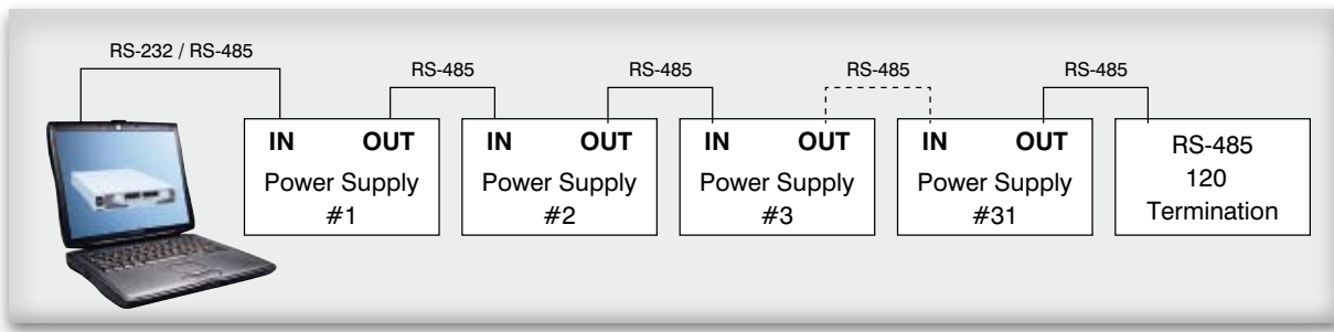
Multi power supplies RS-232 / RS-485 connection
